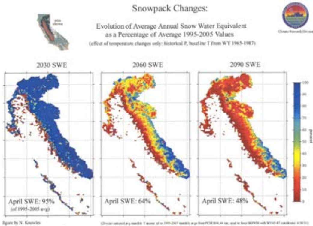
Figure 4 Projected Snow Pack as a percentage of Average 1995-2005 (Knowles and Cayan)
