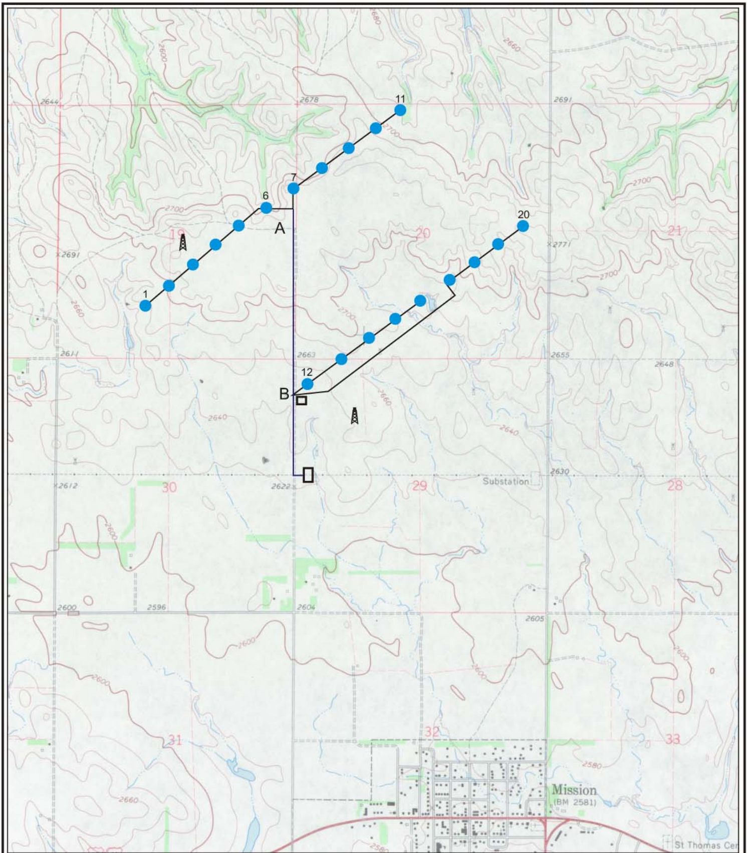
Figure 5 2.5-MW 25-kV Plan WindPACT Turbine Design Scaling Studies National Renewable Energy Project Mission, South Dakota
