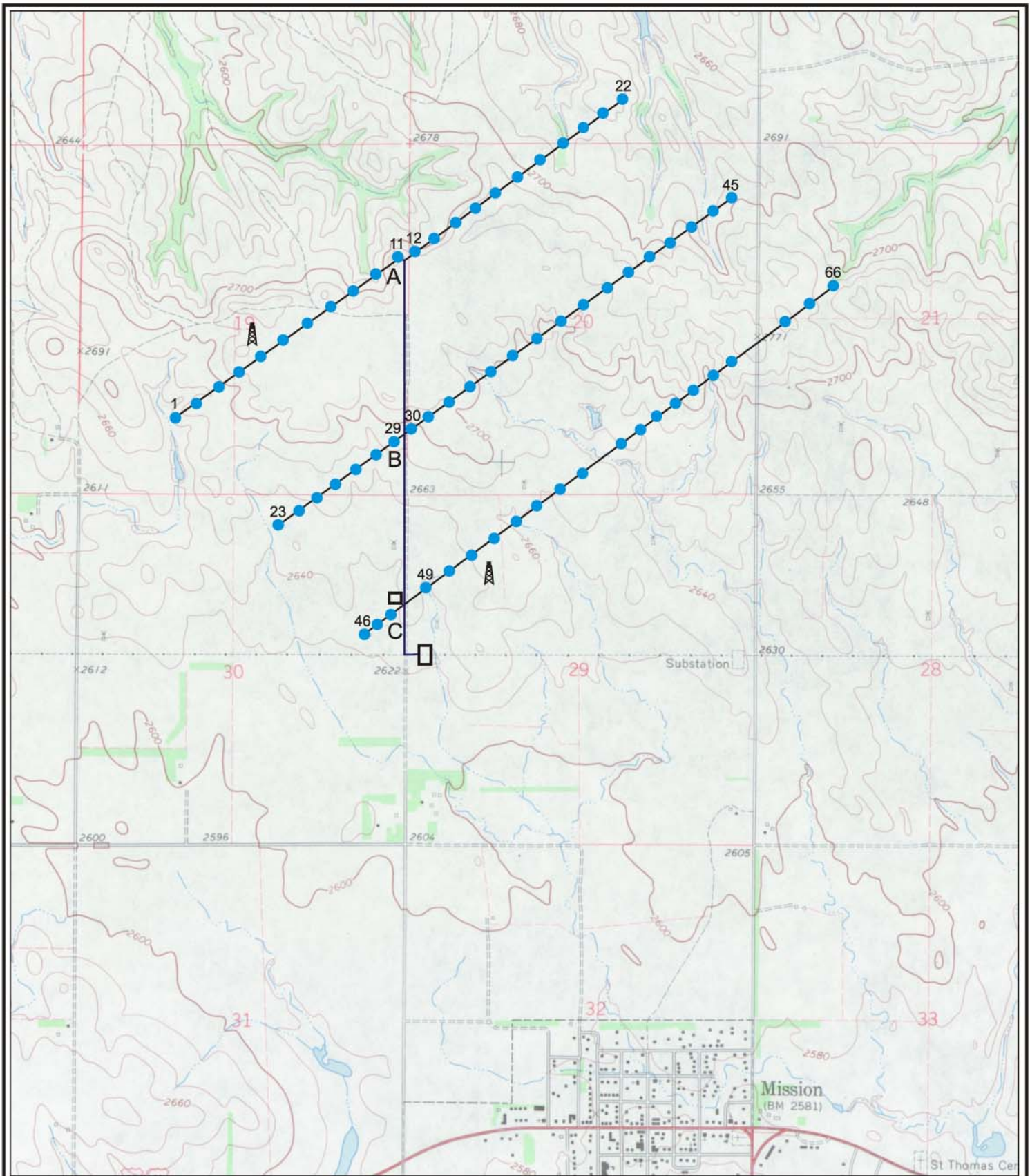
Figure 4 750-kW 25-kV Plan WindPACT Turbine Design Scaling Studies National Renewable Energy Project Mission, South Dakota
