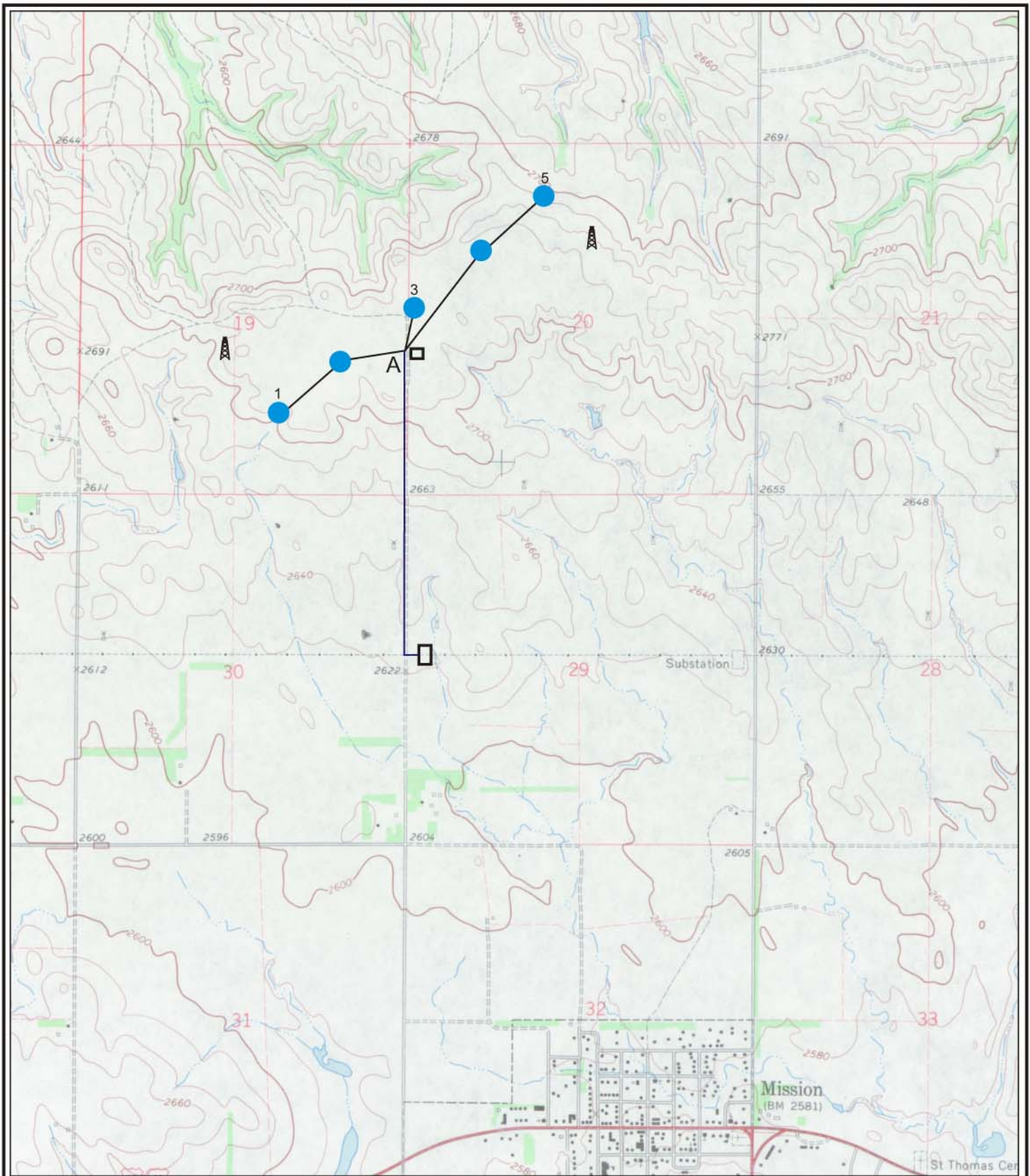
Figure 8 10-MW 25/35-kV Plan WindPACT Turbine Design Scaling Studies National Renewable Energy Project Mission, South Dakota
