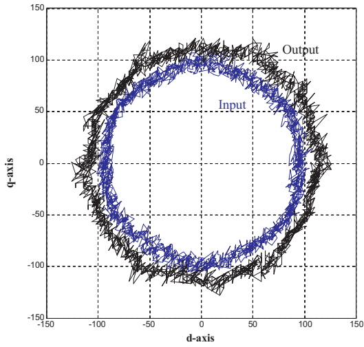
Figure 3.31: Trajectories of input- and output-voltages in dq coordinate
