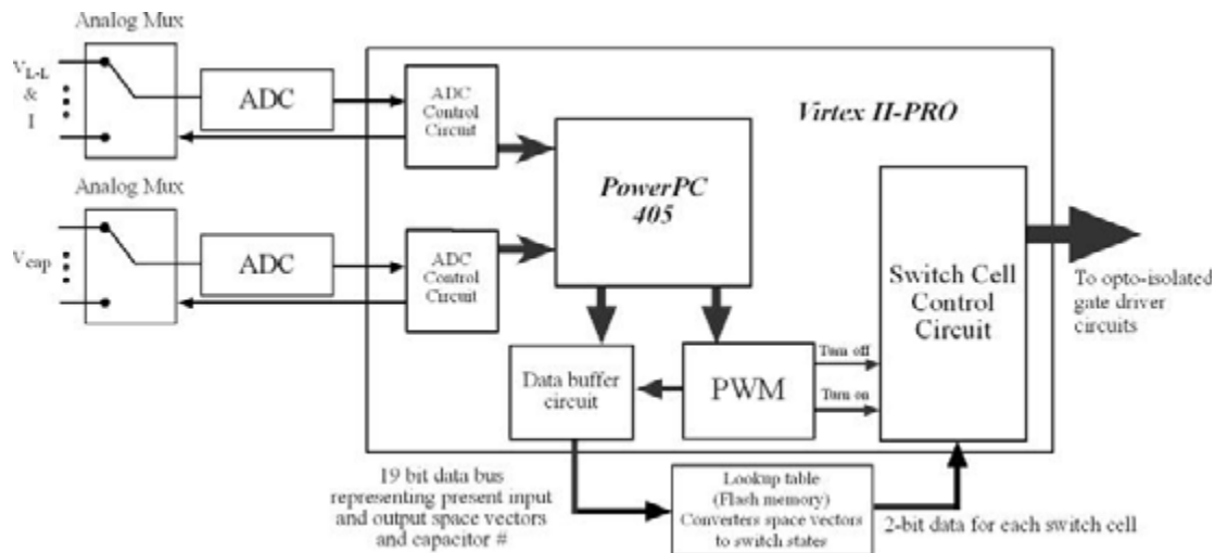
Figure 11.2: Block diagram of the VIRTEX II-PRO FPGA
