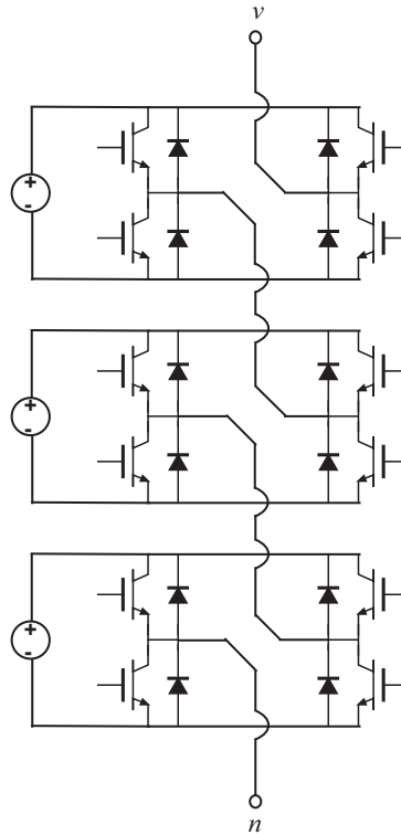
Figure 1.12: One-phase structure of a multilevel converter with H-bridge inverter leg
