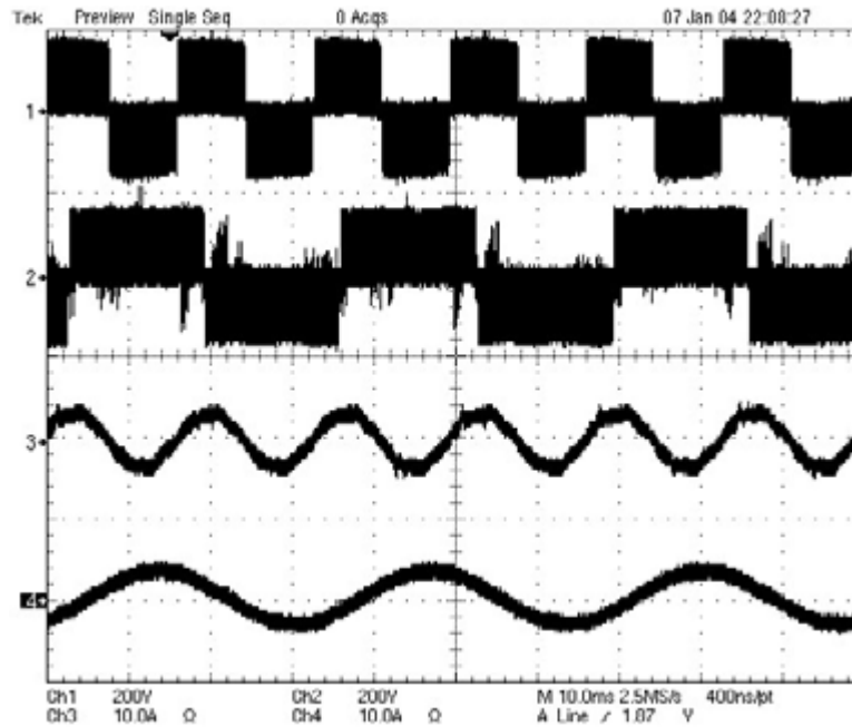
Figure 3.8: Voltage and current waveforms: Trace 1: input PWM line-line voltage waveform at 200 V/div Trace 2: output PWM line-line voltage waveform at 200 V/div Trace 3: input phase current at 10 A/div Trace 4: output phase current at 10 A/div Horizontal scale: 10 ms/div
