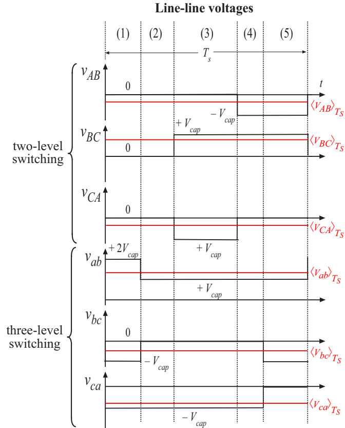
Figure 5.13: The corresponding PWM line-line voltages in the given switching period
