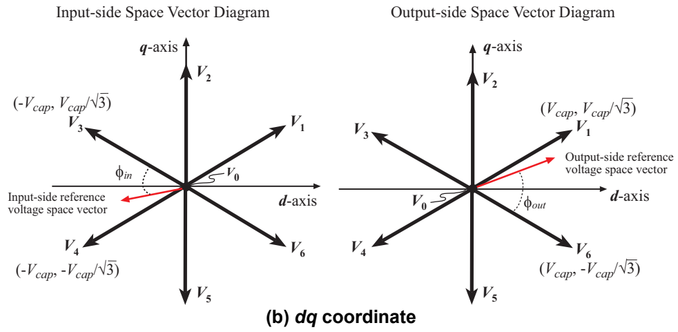
Figure 3.4: An example of SVM
