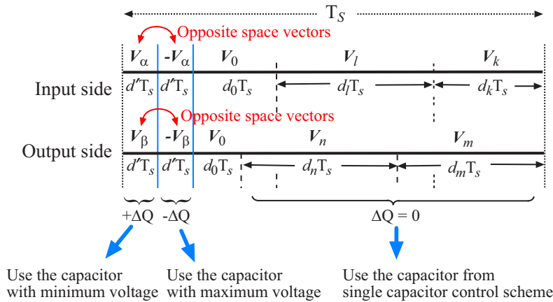
Figure 4.8: Space-vector patterns in each switching period having opposite space vectors at the input and output sides
