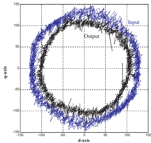
Figure 3.20: Trajectories of input- and output-voltages in dq coordinate
