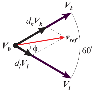
Figure 3.2: Diagram of SVM
