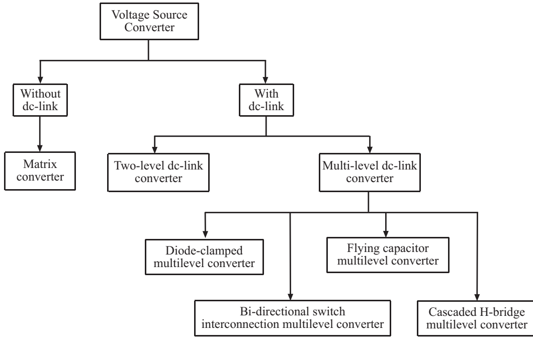
Figure 1.4: Classification of three-phase to three-phase voltage source converter topologies
