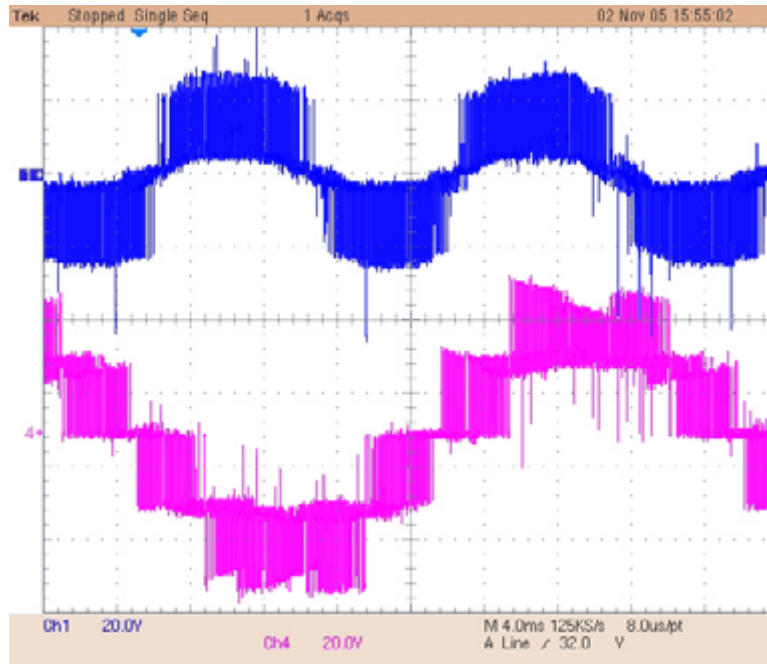
Figure 5.7: Input and output PWM line-line voltage waveforms Trace 1: input line-line voltage with two-level switching Trace 4: output line-line voltage with three-level switching
