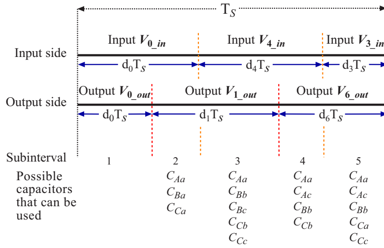
Figure 3.15: Pattern of input-side and output-side space vectors for the example with sets of capacitors that can be used in each subinterval
