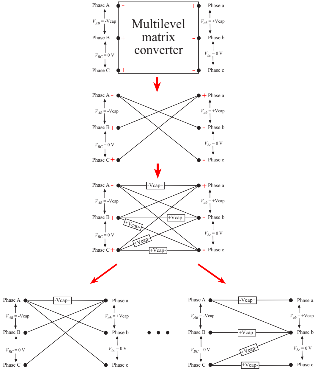
Figure 2.7: Generating valid switching combinations: Case 1
