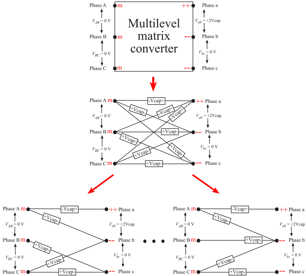
Figure 2.9: Generating valid switching combination: Case 3
