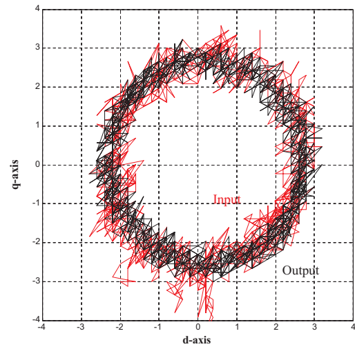
Figure 3.27: Trajectories of input- and output-currents in dq coordinate
