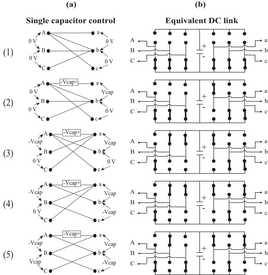
Figure 3.16: Converter configuration with the single-capacitor control technique: (a) switching-device combinations of each subinterval, (b) equivalent DC-link circuits
