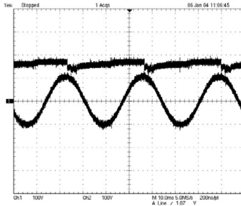
Figure 3.23: Variation of DC capacitor voltages, without any active control Trace 1: DC capacitor voltage waveform Trace 2: filtered load voltage Both traces have scale of 100 V/div
