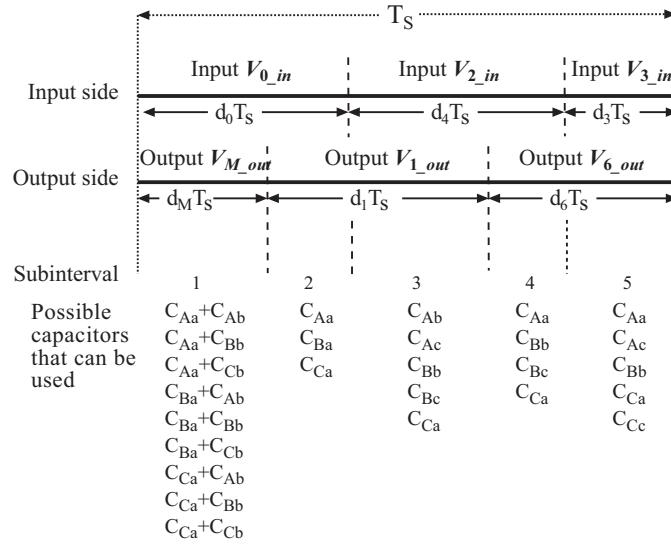
Figure 5.12: Pattern of input and output space vectors for the example with sets of capacitors that can be used in each subinterval
