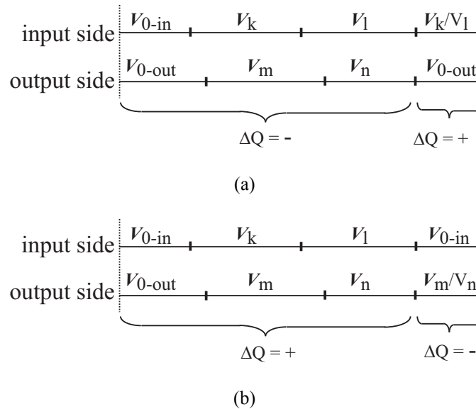
Figure 4.3: Space-vector pattern for regulating capacitor voltages: (a) for charging capacitor, (b) for discharging capacitor
