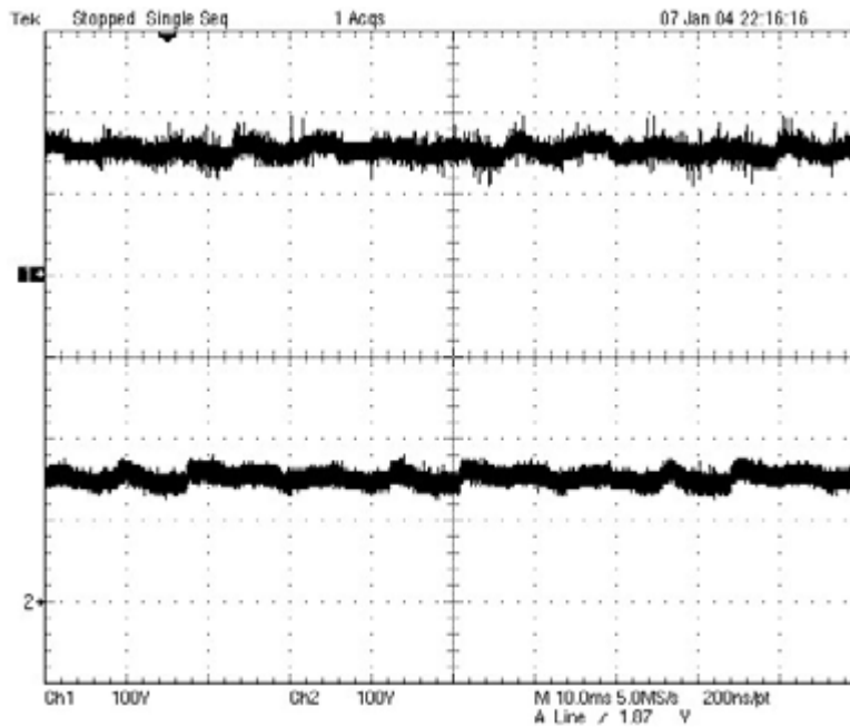
Figure 3.13: The DC capacitor voltage waveforms of two different switch cells; Trace 1 and Trace 2 are both set to scale of 100 V/div at different ground reference level
