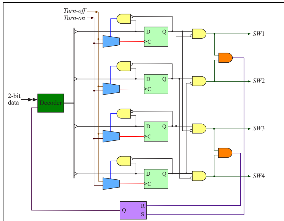
Figure 6.16: Block diagram of the switch-cell controller circuit
