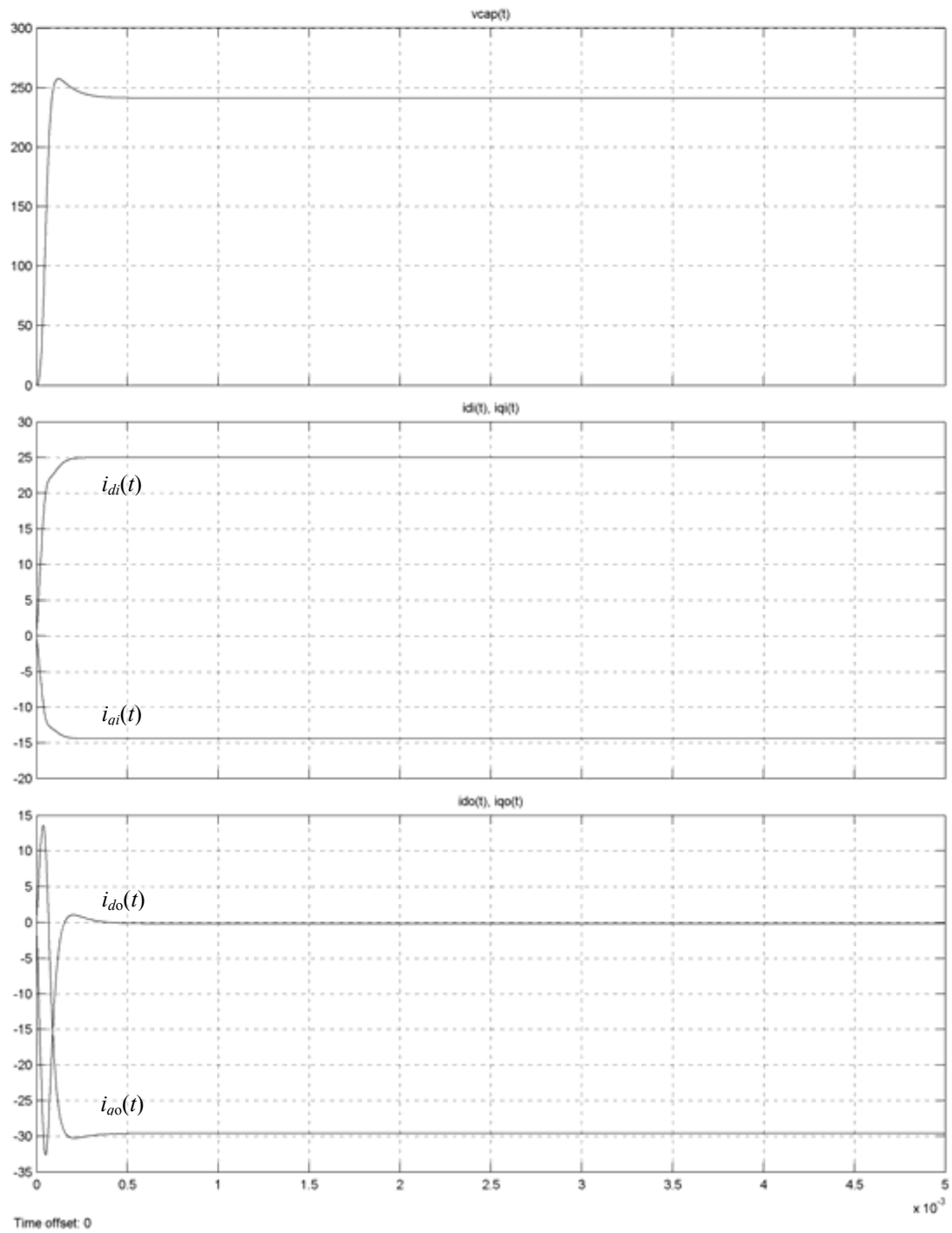
Figure 10.14: Simulation results for the following operating point: Input side: 240 V, 13 Hz, unity power factor Output side: 240 V, 60 Hz, 20 A, 0.5 power factor The first part is the capacitor voltage response, the second part is the input dq currents responses, and the third part is the output dq currents responses
