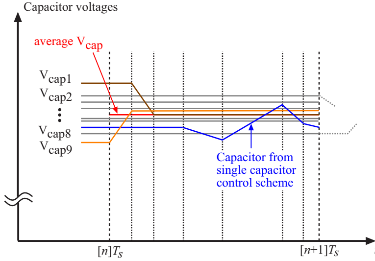
Figure 4.10: The ideal capacitor voltage waveforms for the proposed capacitor voltage-balancing scheme
