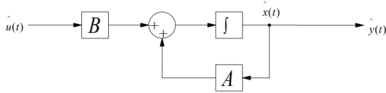
Figure 9.4: Block diagram of the linearized converter's state-space equations
