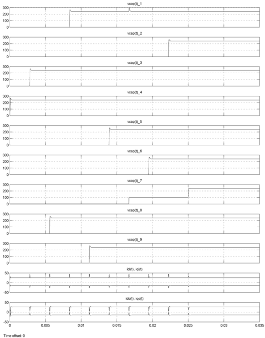
Figure 10.17: Simulation results for the following operating point: Input side: 240 V, 25 Hz, unity power factor Output side: 240 V, 60 Hz, 20 A, unity power factor The first nine parts are the capacitor voltages responses, the tenth part is the input dq currents responses, and the last part is the output dq currents responses
