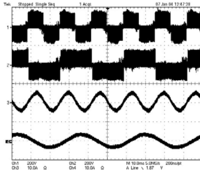
Figure 3.30: Voltage and current waveforms, Case 3 Trace 1: input line-line PWM voltage waveform at 200 V/div Trace 2: output-side line-line PWM voltage waveform at 200 V/div Trace 3: input phase current at 10 A/div Trace 4: output phase current at 10 A/div Horizontal scale: 10 ms/div
