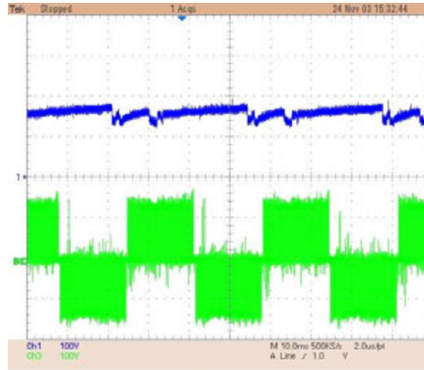
Figure 4.11: Waveforms of a capacitor voltage and an output PWM line-line voltage without capacitor voltage regulation
