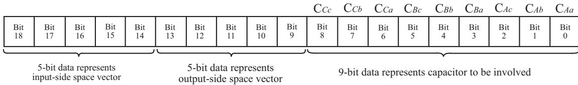
Figure D.1: Assignment of bits for the address of the flash memory.
