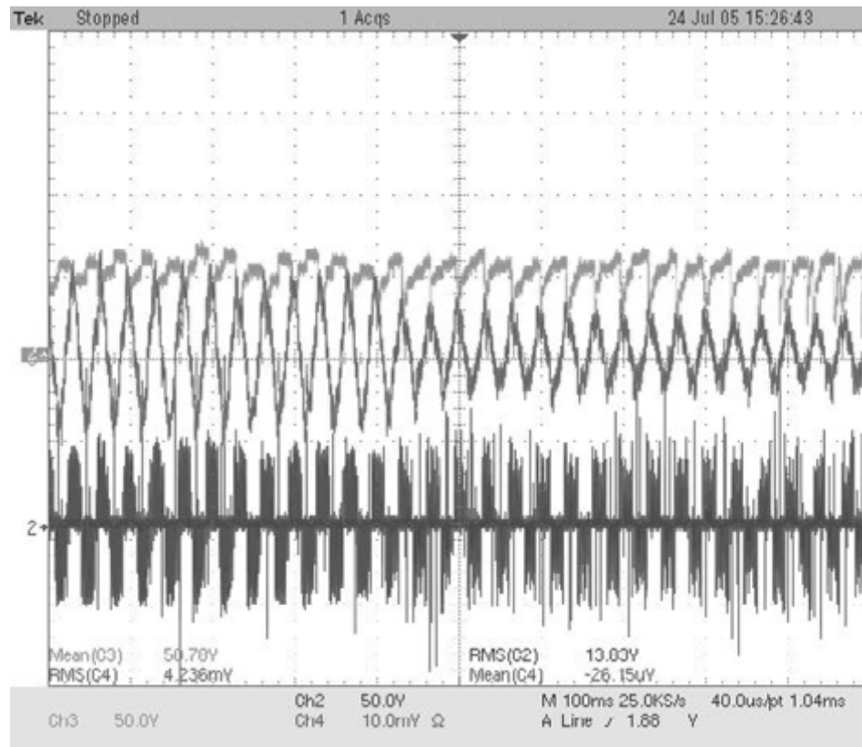
Figure 11.3: Experimental results of the matrix converter prototype when the output-line current changes from 1 A to 0.5 A amplitude:
