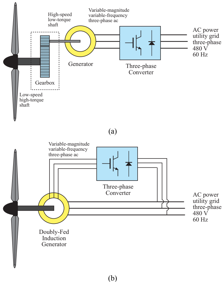
Figure 1.3: Variable-speed wind turbine configurations: (a) with full-scale converter, (b) with reduced VA converter
