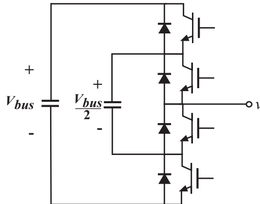
Figure 1.11: Switching device configuration for one phase of a three-level flying capacitor converter
