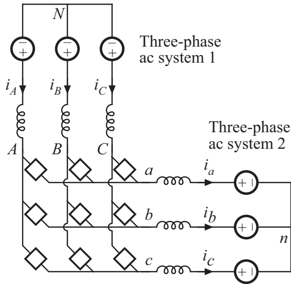
Figure 2.1: Basic configuration of a multilevel matrix converter
