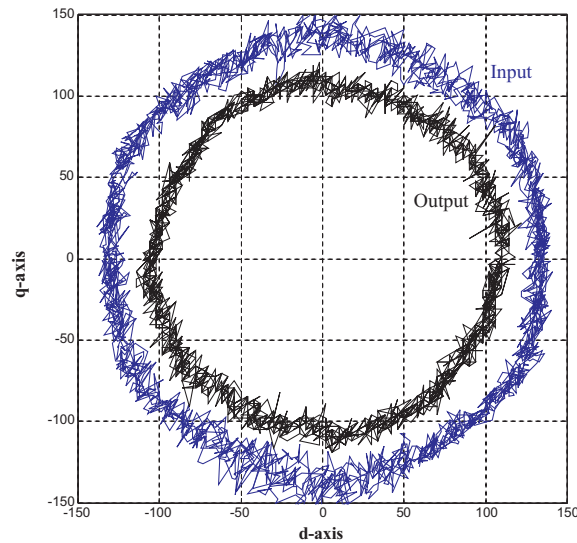
Figure 3.9: Trajectories of input- and output-voltages in dq coordinate
