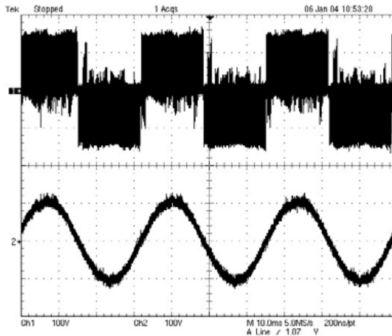
Figure 3.22: The 30-Hz output line-line voltage waveforms for Case 1 Trace 1: PWM voltage waveform at the output of the switch network Trace 2: load voltage waveform after filtered by LC output low-pass network
