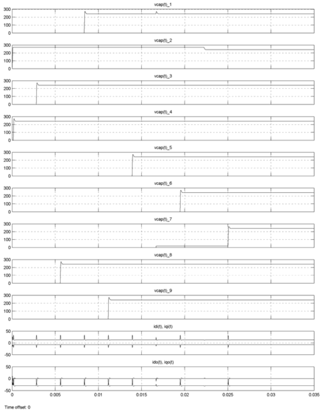
Figure 10.18: Simulation results for the following operating point: Input side: 240 V, 25 Hz, unity power factor Output side: 240 V, 60 Hz, 20 A, 0.5 power factor The first nine parts are the capacitor voltages responses, the tenth part is the input dq currents responses, and the last part is the output dq currents responses
