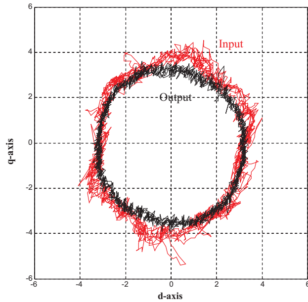
Figure 3.10: Trajectories of input and output currents in dq coordinate
