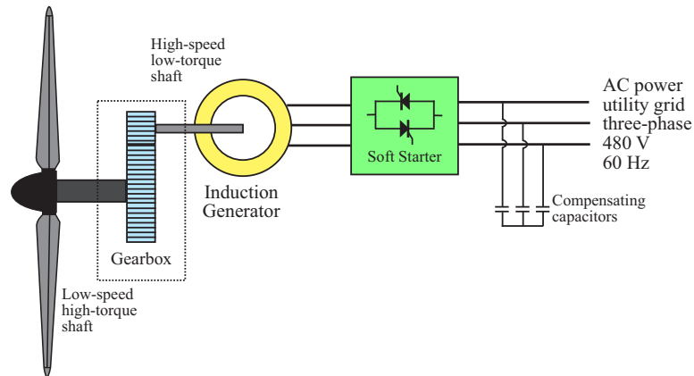
Figure 1.2: Constant-speed wind turbine configuration with a squirrel-cage induction generator that is directly coupled to the grid
