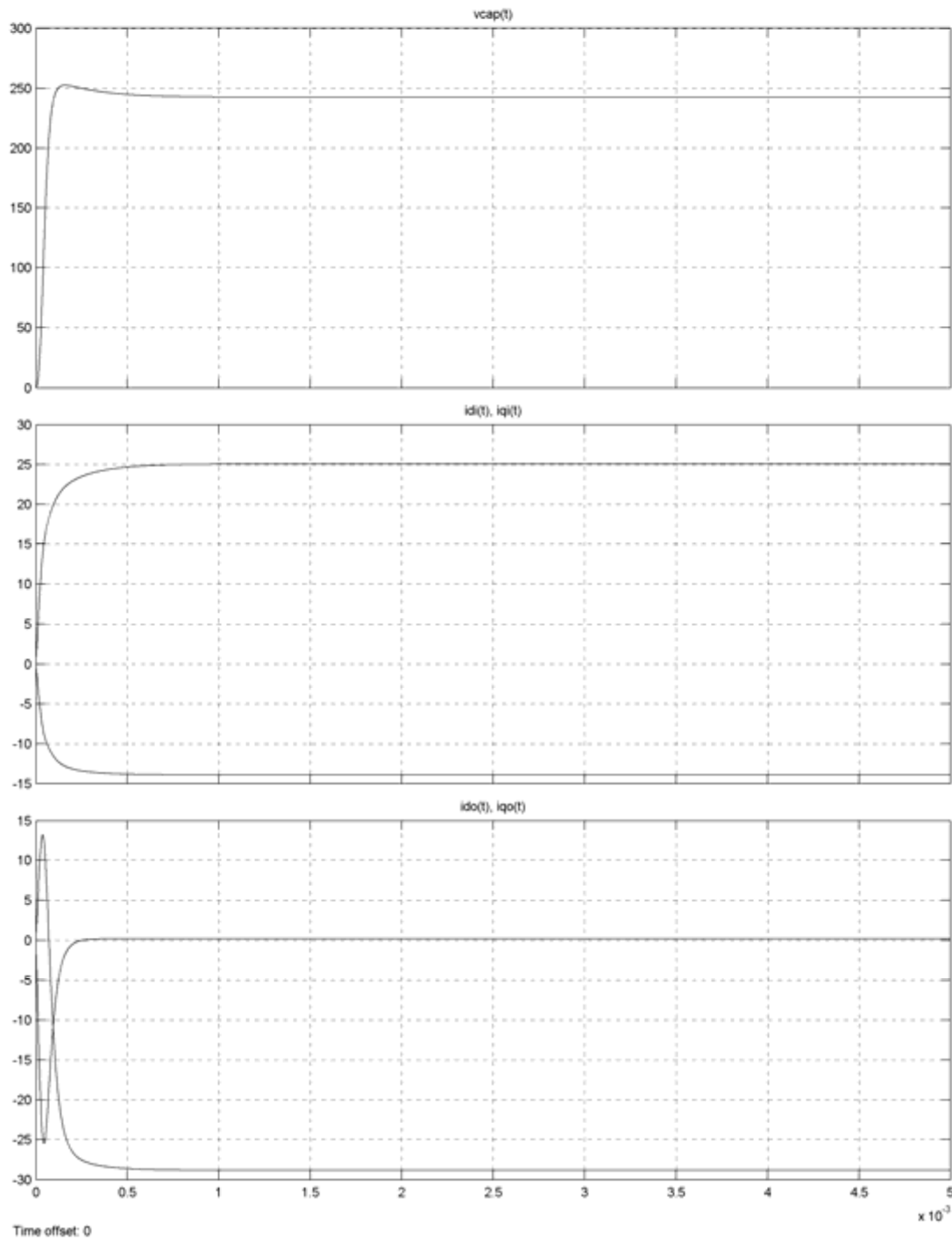
Figure 10.8: Simulation results for the following operating point: Input side: 240 V, 13 Hz, unity power factor Output side: 240 V, 60 Hz, 20 A, 0.5 power factor The first part is the capacitor voltage response, the second part is the input dq currents responses, and the third part is the output dq currents responses
