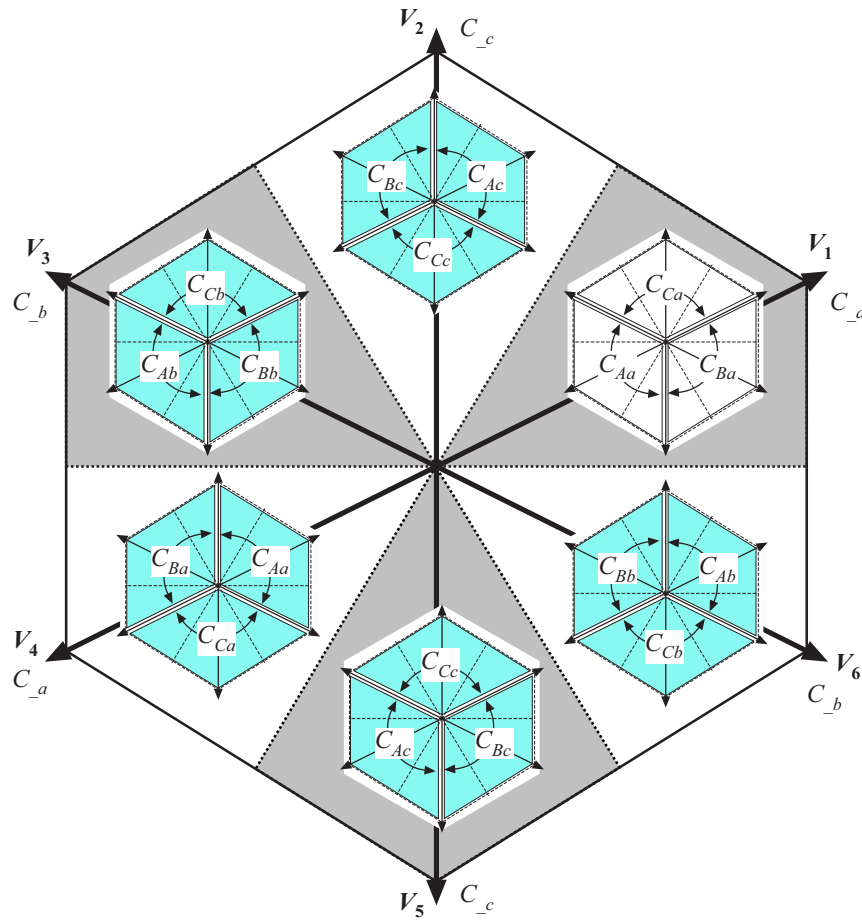
Figure 3.17: Summary of switch-cell capacitor choice with the single-capacitor control scheme for the case of d_{0\_out} < d_{0\_in}
