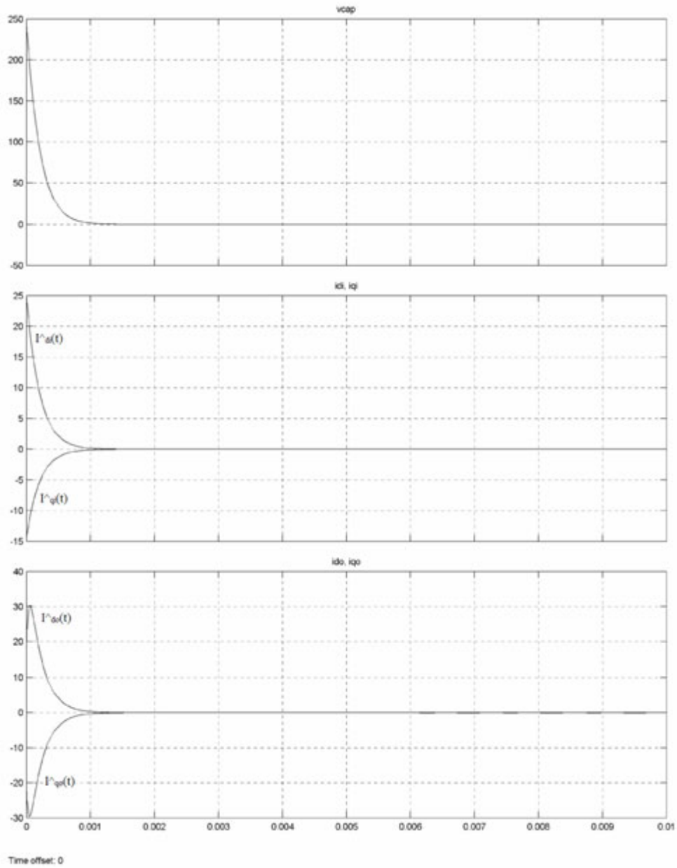
Figure 10.3: Simulation results of the closed-loop linearized state-space model of the matrix converter when a pole-placement controller is used
