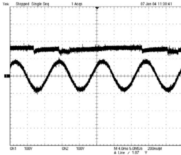
Figure 3.29: Variation of DC capacitor voltage, without active control Trace 1: DC capacitor voltage waveform Trace 2: filtered load voltage waveform Both traces have scale of 100 V/div
