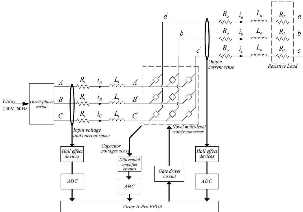
Figure 11.1: Block diagram of the prototype matrix converter
