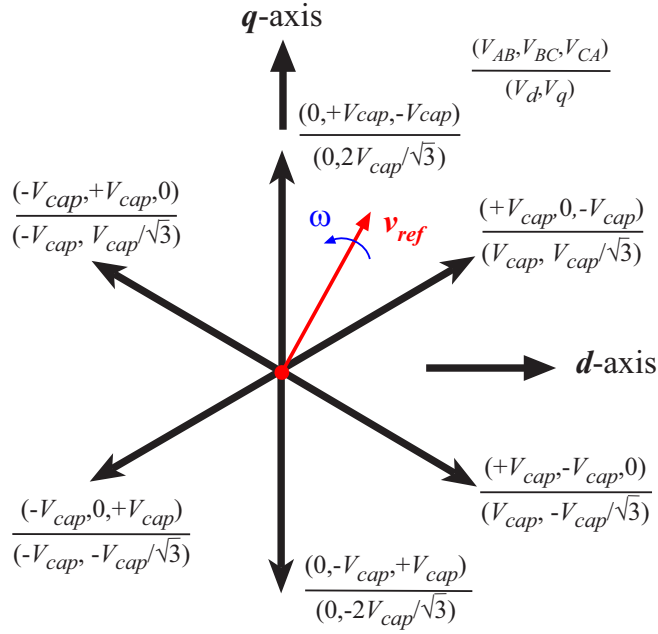
Figure 4.4: Seven space vectors employed in the two-level switching
