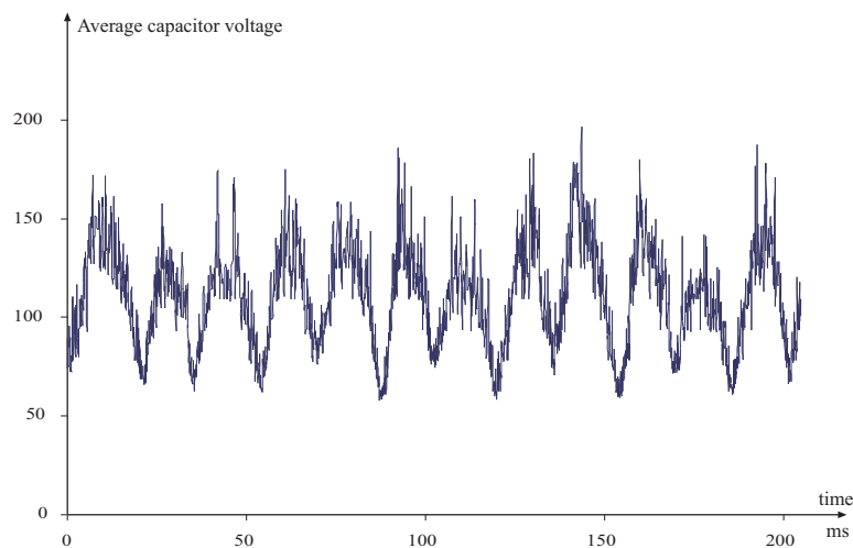
Figure 4.15: Waveform of the average of nine capacitor voltages
