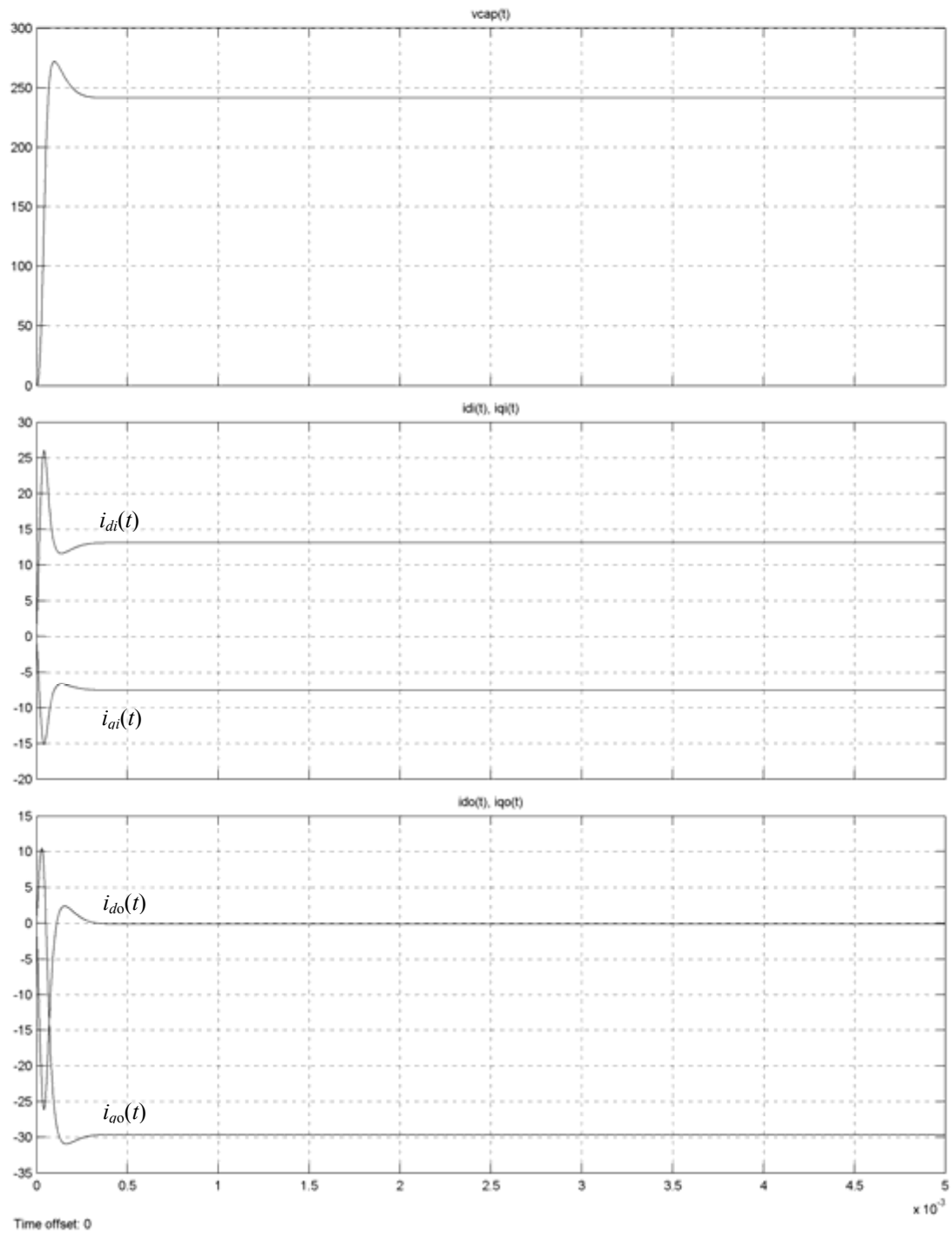
Figure 10.12: Simulation results for the following operating point: Input side: 240 V, 25 Hz, unity power factor Output side: 240 V, 60 Hz, 20 A, 0.5 power factor The first part is the capacitor voltage response, the second part is the input dq currents responses, and the third part is the output dq currents responses
