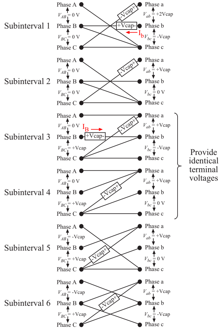
Figure 5.14: Example of switching-device combinations to balance charge of the capacitor C_{Bb}
