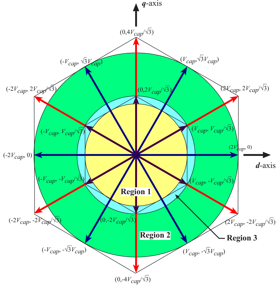
Figure 1.15: Operating regions of the multilevel matrix converter in dq diagram
