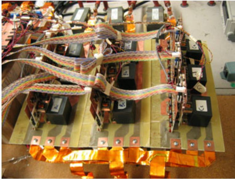
Figure 6.3: Power stage consisting of three printed circuit boards; each PCB contains three H-bridge switch cells
