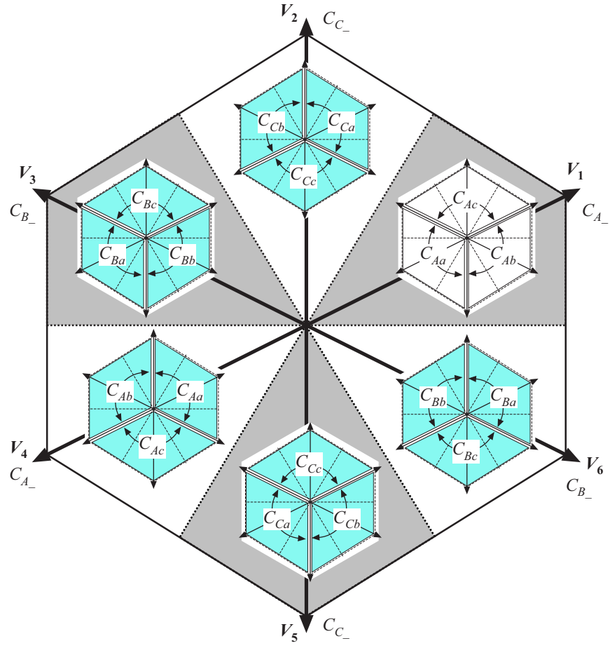
Figure 3.18: Summary of switch-cell capacitor choice with the single-capacitor control scheme for the case of d_{0\_out} > d_{0\_in}
