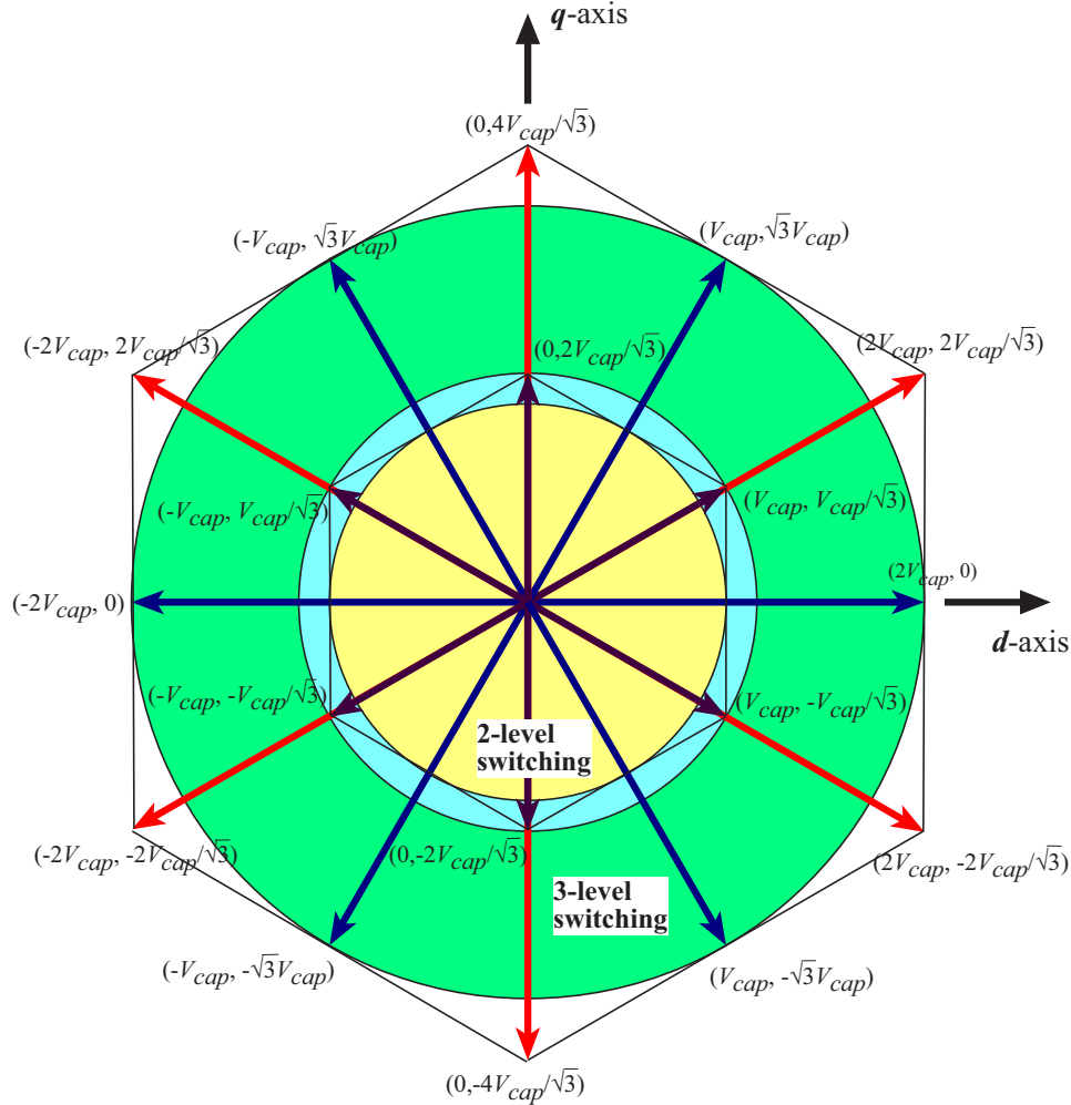
Figure 5.2: Operating regions of the multilevel matrix converter in dq diagram
