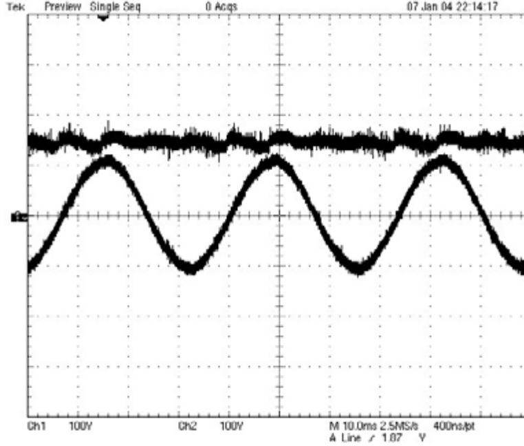
Figure 3.12: Variation of DC capacitor voltage, without active control Trace 1: DC capacitor voltage waveform Trace 2: filtered-load voltage waveform Both traces have scale of 100 V/div
