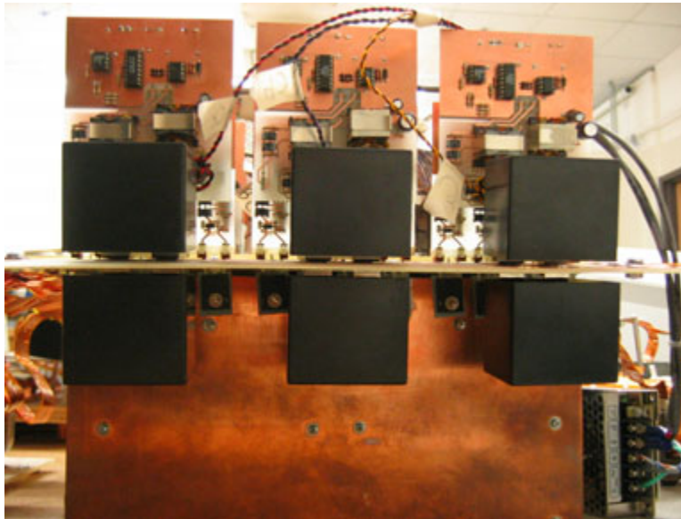
Figure 6.4: Three H-bridge switch cells per PCB
