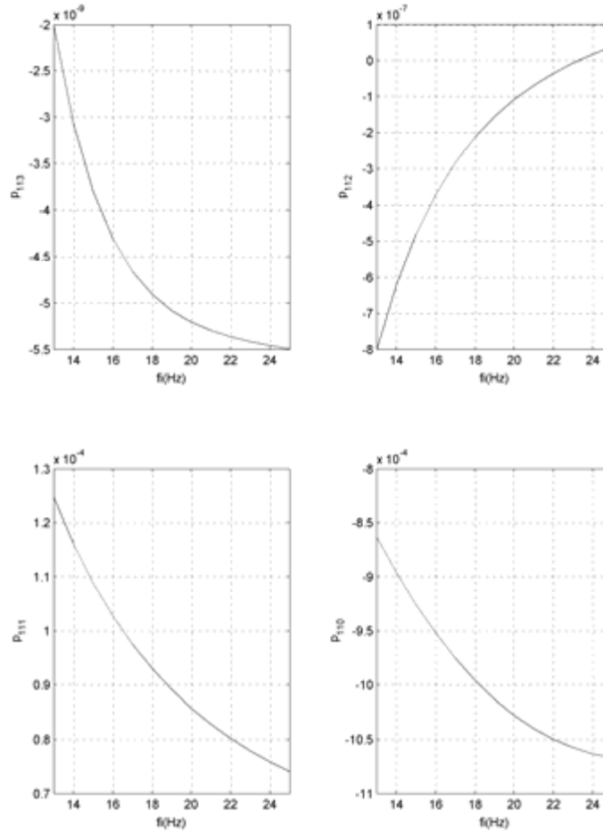
Figure 10.16: Plots of the coefficients p_{11x} ( x = 0-3 ) as a function of the input-line frequency
