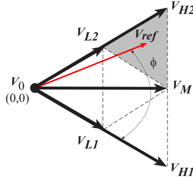
Figure 5.5: SVM for three-level switching, Case 3
