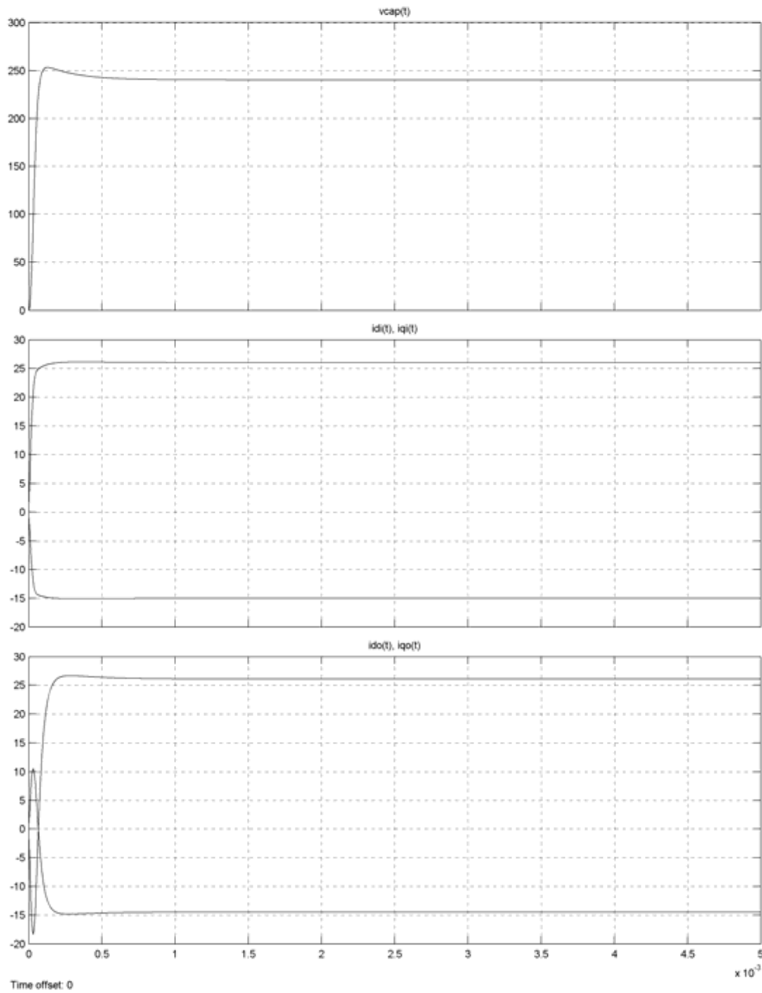
Figure 10.5: Simulation results for the following operating point: Input side: 240 V, 25 Hz, unity power factor Output side: 240 V, 60 Hz, 20 A, unity power factor The first part is the capacitor voltage response, the second part is the input dq currents responses, and the third part is the output dq currents responses
