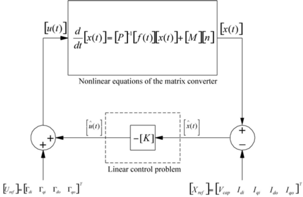
Figure 10.4: Implementation of the linear controller in the nonlinear model of the matrix converter
