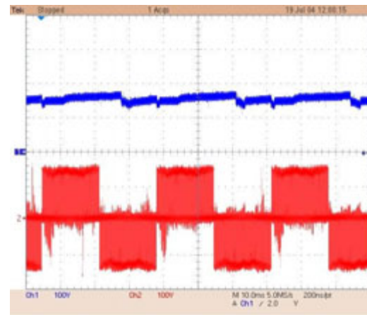
Figure 4.2 Capacitor voltage and output PWM line-line voltage waveforms when with the converter operated at the switching frequency of 25 kHz
