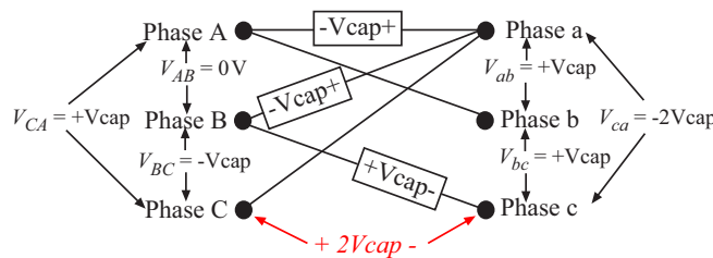
Figure 2.6: An example of invalid switching-device combination having 2V_{cap} across the non-conducting switch cells
