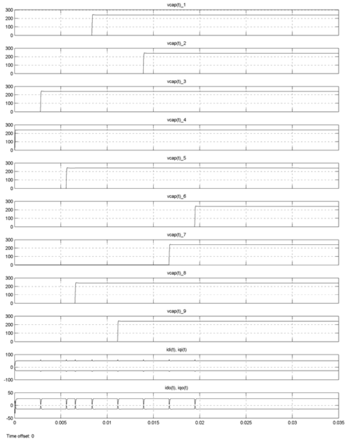
Figure 10.19: Simulation results for the following operating point: Input side: 240 V, 13 Hz, unity power factor Output side: 240 V, 60 Hz, 20 A, unity power factor The first nine parts are the capacitor voltages responses, the tenth part is the input dq currents responses, and the last part is the output dq currents responses
