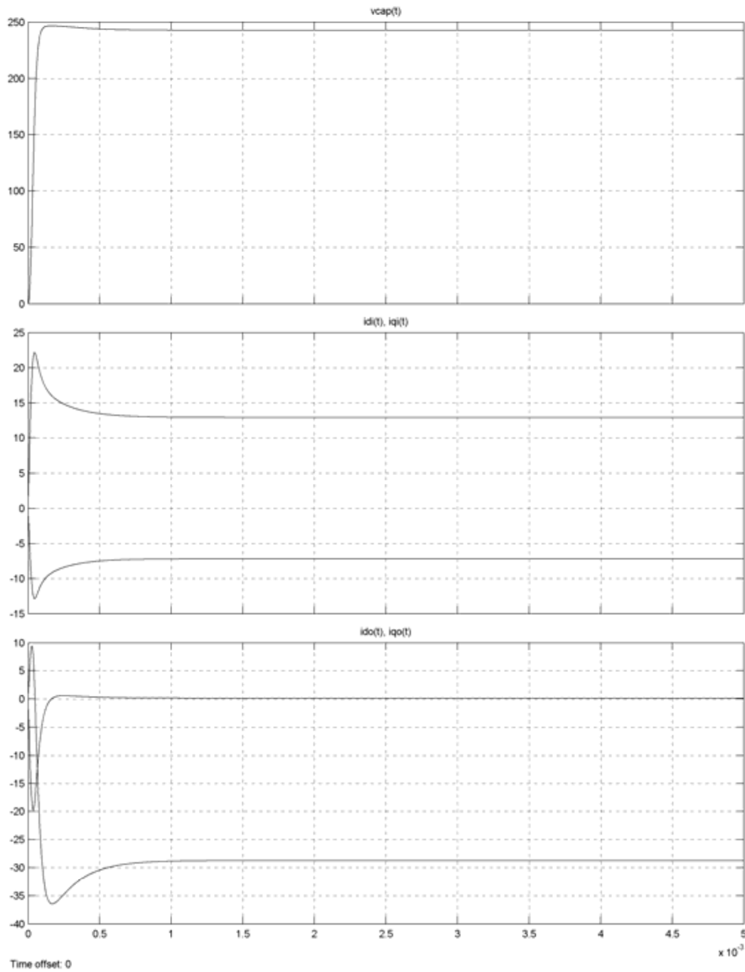
Figure 10.6: Simulation results for the following operating point: Input side: 240 V, 25 Hz, unity power factor Output side: 240 V, 60 Hz, 20 A, 0.5 power factor The first part is the capacitor voltage response, the second part is the input dq currents responses, and the third part is the output dq currents responses
