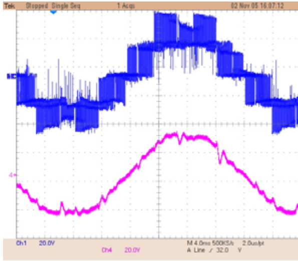
Figure 5.9: Waveforms of output PWM in-line voltage and the filtered output line-line voltage
