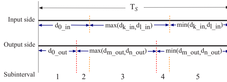
Figure 3.14: The pattern of input-side and output-side space vectors for the single-capacitor control scheme
