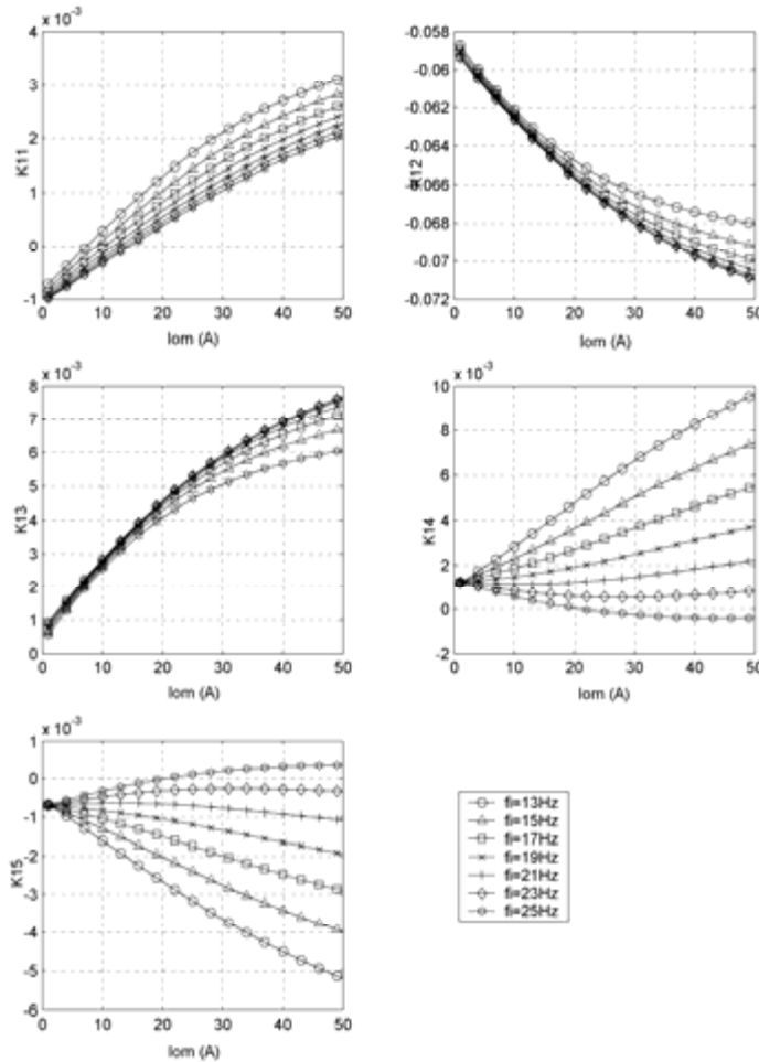
Figure 10.15: Plots of the first row of the optimal controller-gain matrix as a function of the output current amplitude, plotted for various input-line frequencies.
