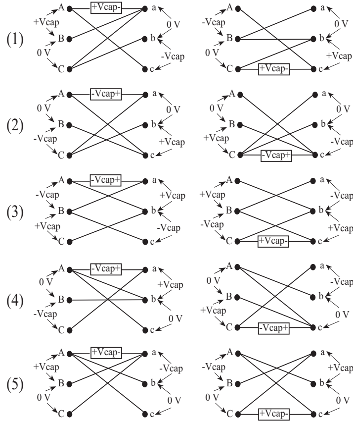
Figure 4.9: Example of switching-device combinations that involve capacitors C_{Aa} and C_{Cc}
