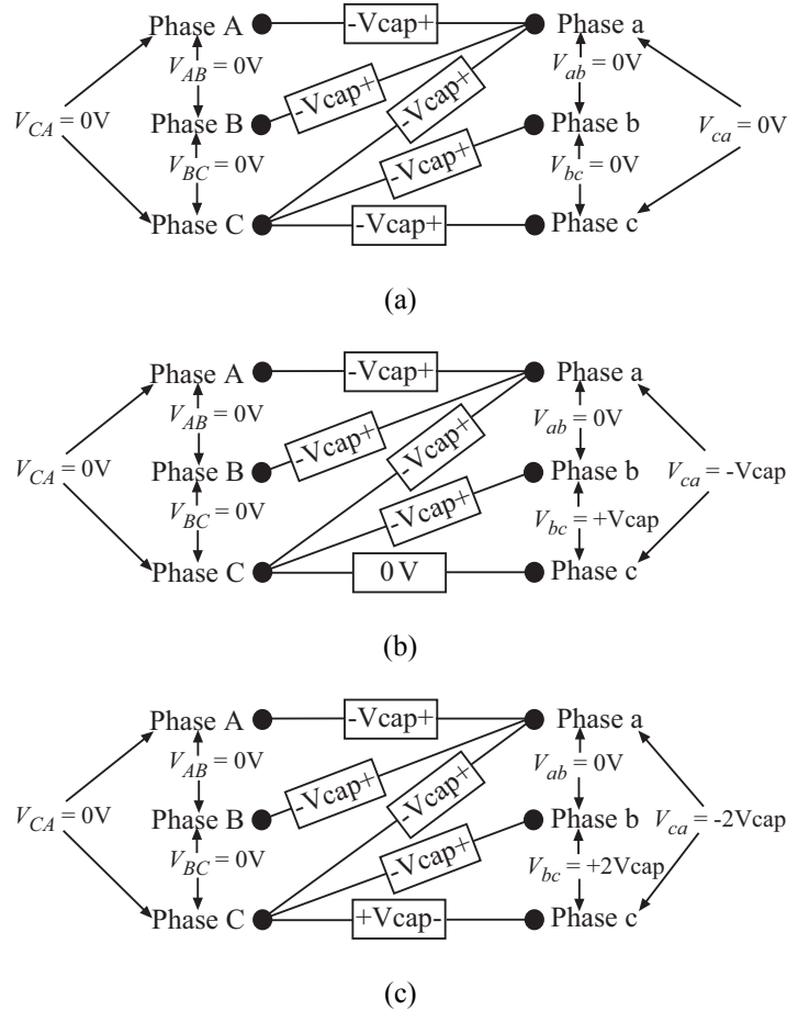
Figure 2.5: Examples of different switching-device combinations in the multilevel matrix converter
