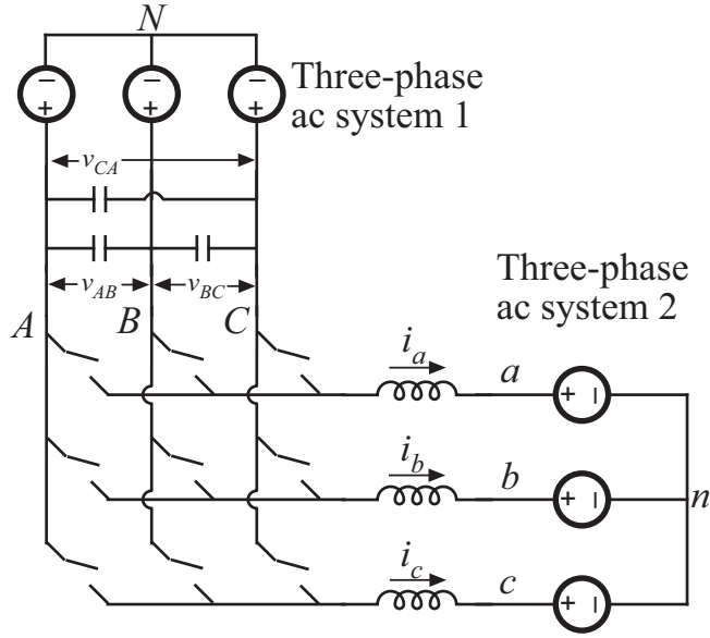
Figure 1.5: Conventional matrix converter topology
