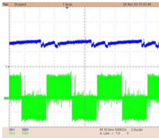
Figure 4.1: Capacitor voltage and output PWM line-line voltage waveforms when the converter operated at the switching frequency of 50 kHz
