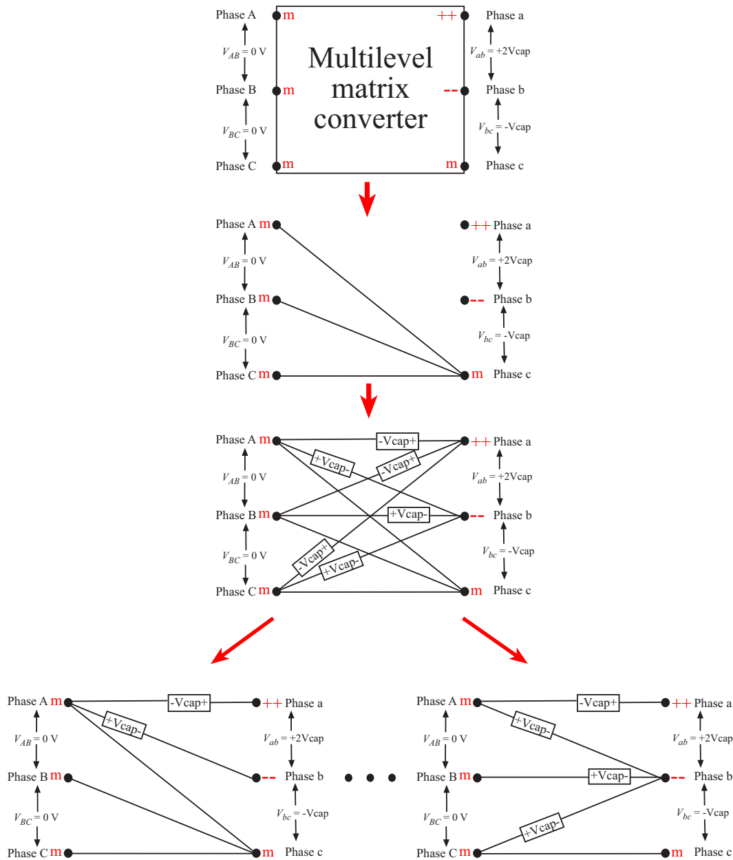
Figure 2.8: Generating valid switching combination: Case 2
