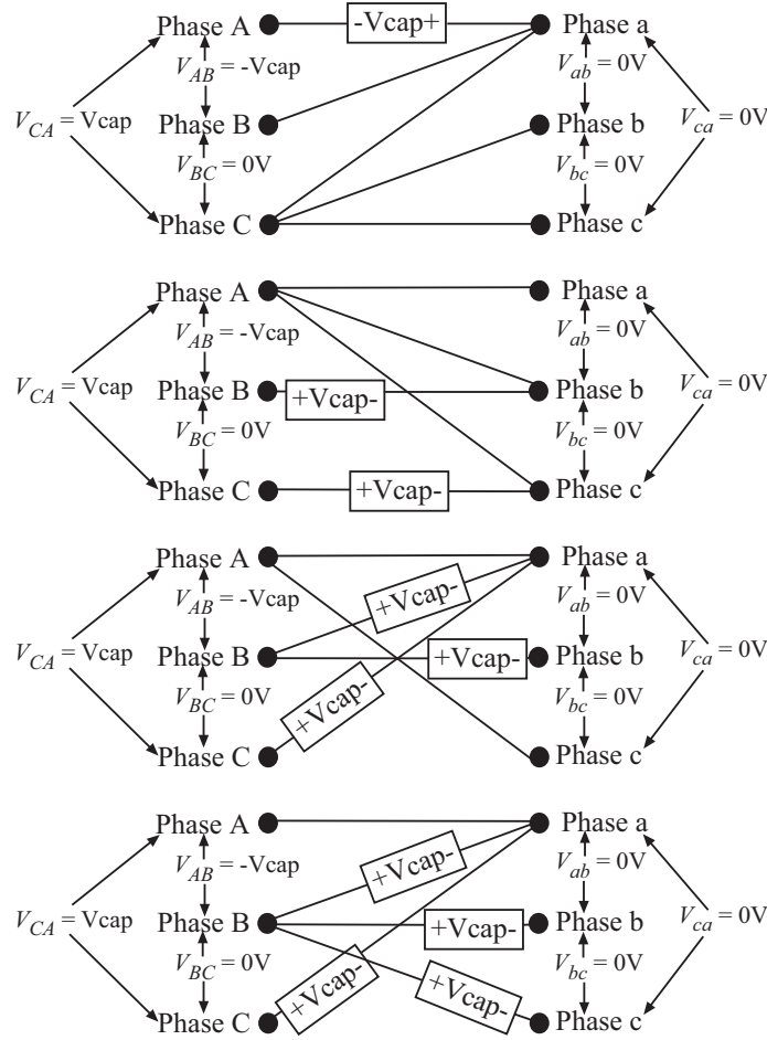
Figure 2.10: Examples of redundant switch combinations
