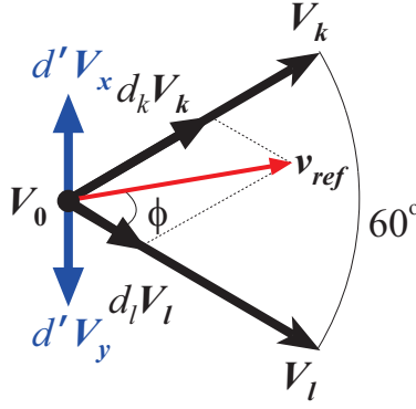
Figure 4.6: Modified SVM
