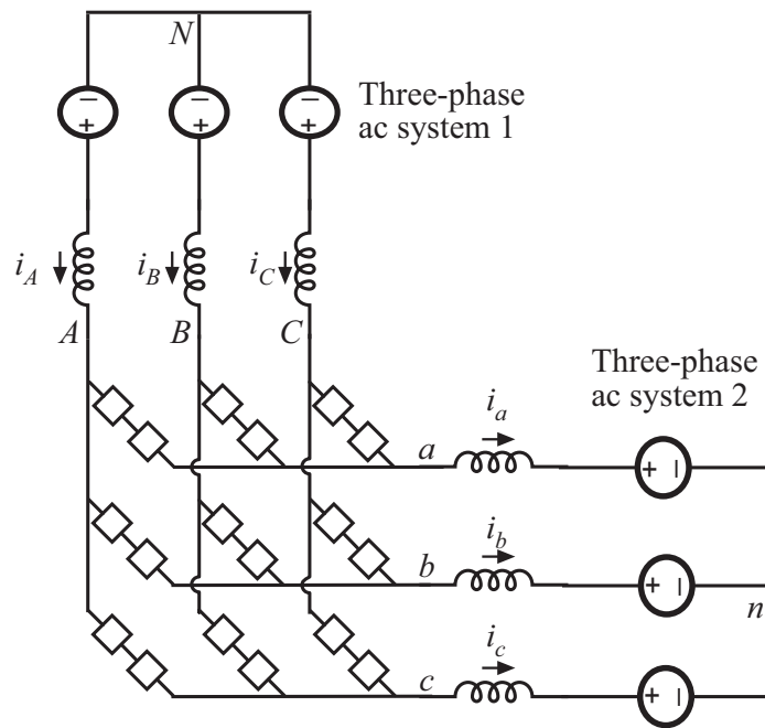
Figure 2.3: A multilevel matrix converter containing two of the switch cells in each branch to increase voltage-levels
