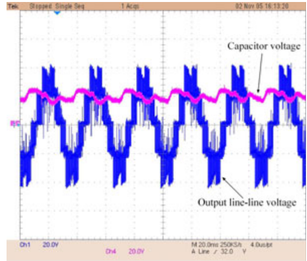
Figure 5.10: Output line-line voltage and capacitor voltage waveforms
