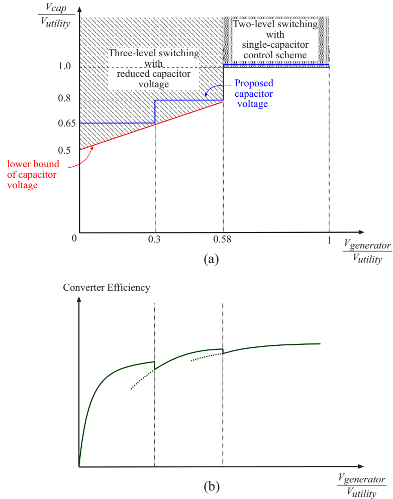
Figure 1.16: (a) Proposed capacitor voltage of the multilevel matrix converter in the wind turbine system, (b) prospective converter efficiency
