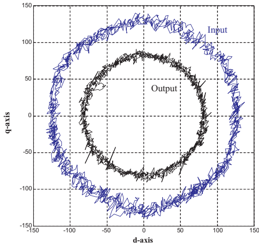
Figure 3.26: Trajectories of input- and output-voltages in dq coordinate
