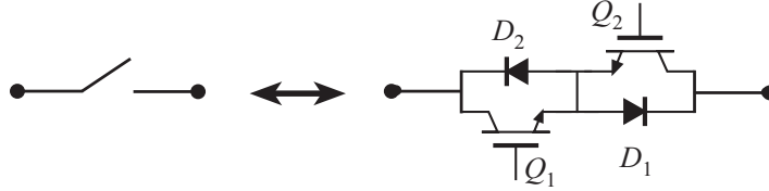
Figure 1.6: Conventional four-quadrant switch used in the matrix converter
