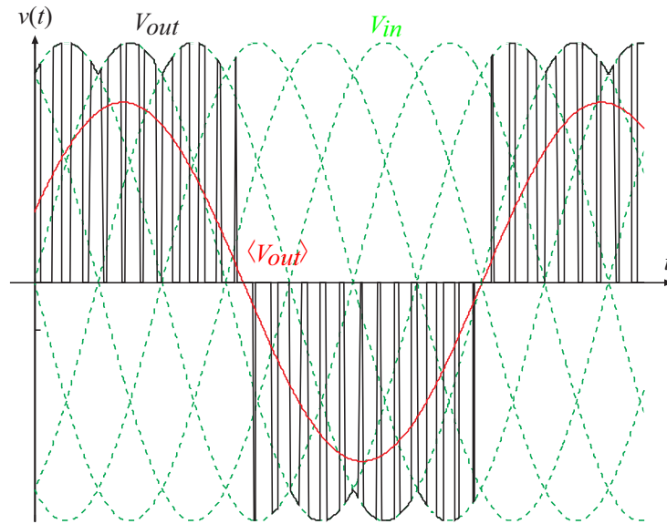
Figure 1.7: Output voltage waveform generated from matrix converter using the SVM technique
