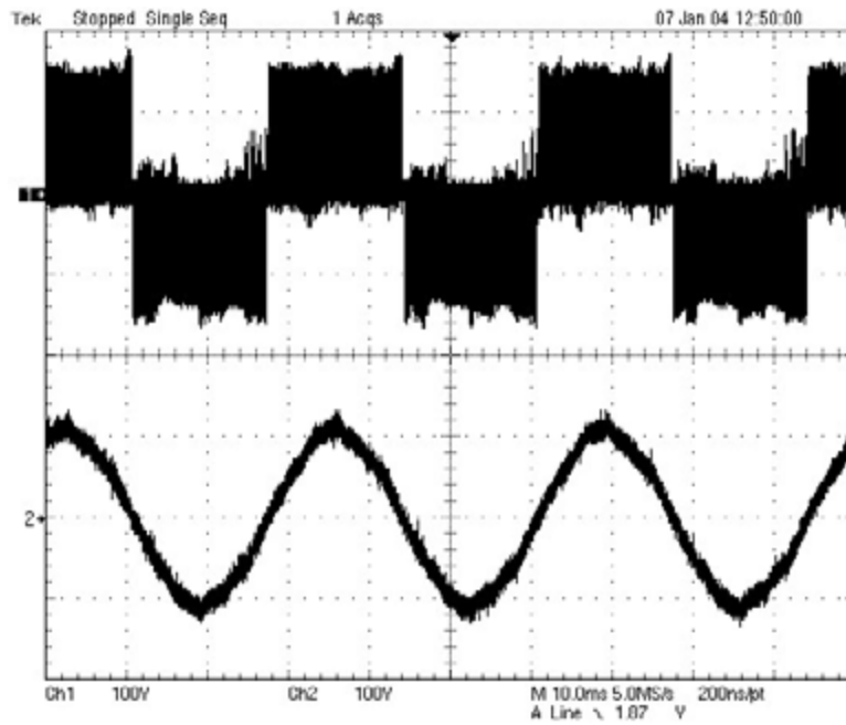
Figure 3.33: The 30-Hz output line-line voltage waveforms for Case 3 Trace 1: PWM voltage waveform at the output of the switch network Trace 2: load voltage waveform after filtered by LC output low-pass network
