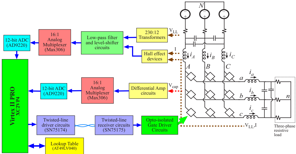
Figure 6.1: Block diagram for the laboratory prototype of multilevel matrix converter
