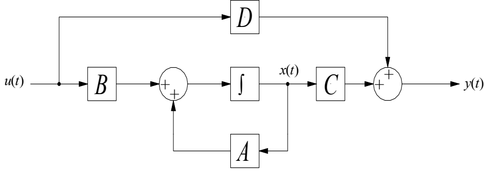
Figure 9.3: Block diagram of a general LTI state space model.
