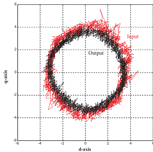
Figure 3.21: Trajectories of input- and output-currents in dq coordinate
