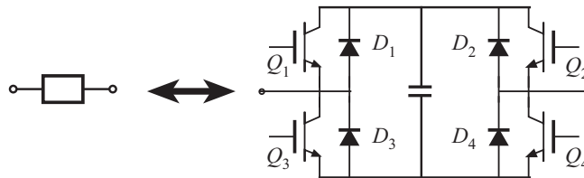
Figure 2.2: Schematic diagram of an H-bridge capacitor clamped switch cell
