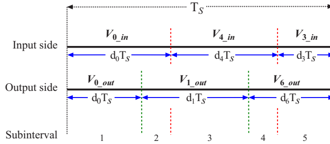
Figure 3.5: Possible switching pattern of the input and the output space vectors in one switching period for the example
