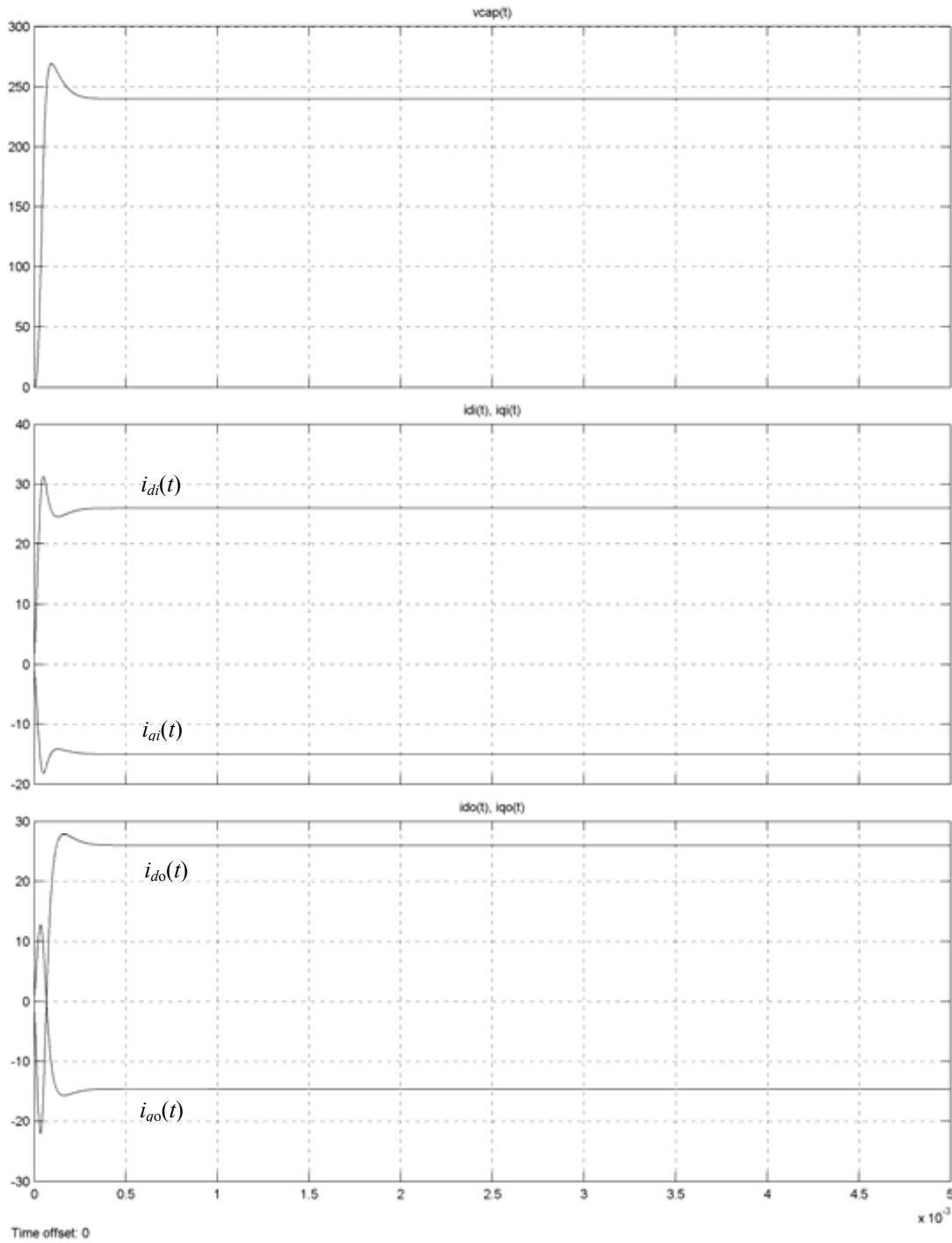
Figure 10.11: Simulation results for the following operating point: Input side: 240 V, 25 Hz, unity power factor Output side: 240 V, 60 Hz, 20 A, unity power factor The first part is the capacitor voltage response, the second part is the input dq currents responses, and the third part is the output dq currents responses
