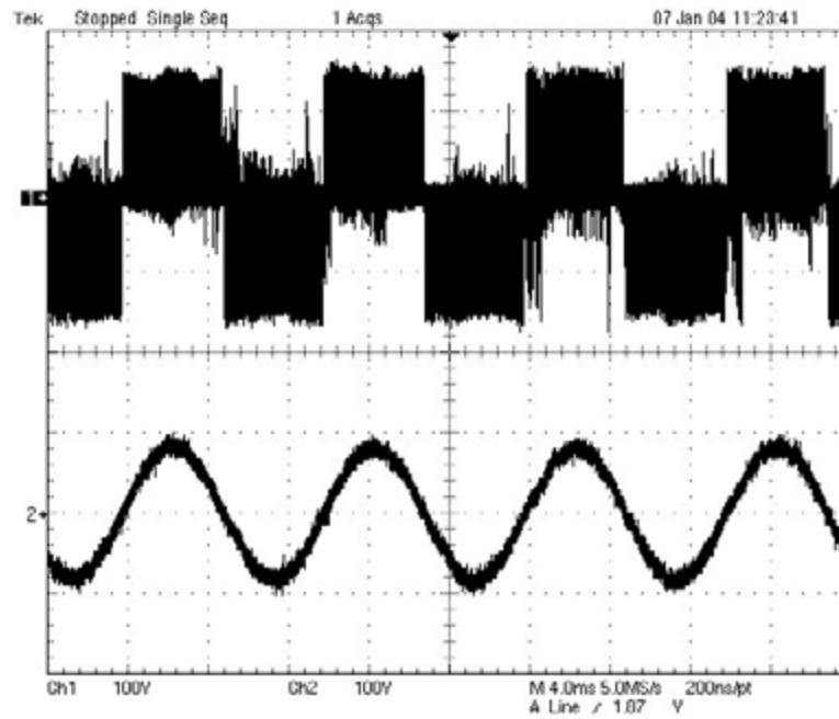
Figure 3.28: The 100-Hz output line-line voltage waveforms for Case 2 Trace 1: PWM voltage waveform at the output of the switch network Trace 2: load voltage waveform after filtered by LC output low-pass network
