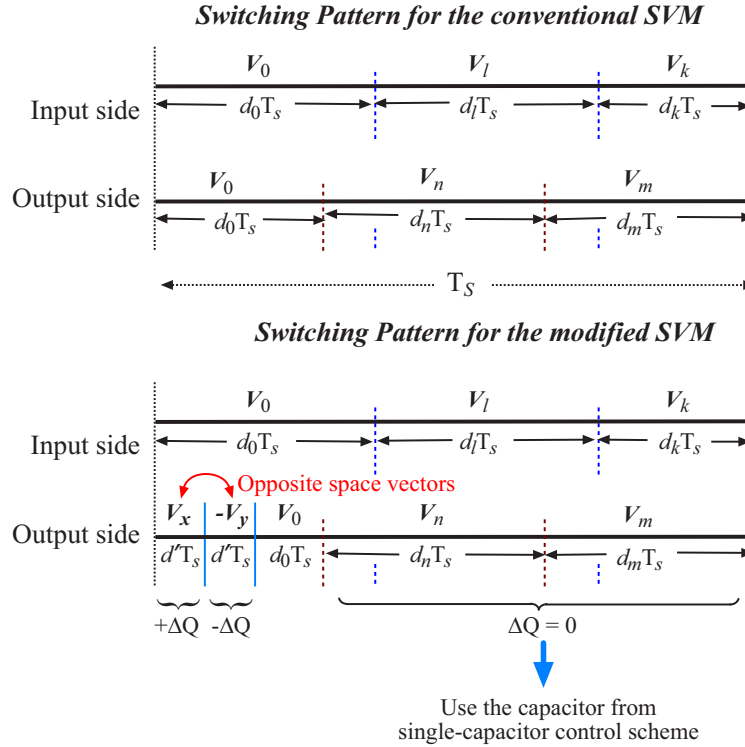
Figure 4.7: Space vector patterns with the opposite space vectors at the output side
