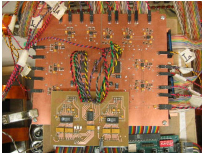
Figure 6.11: Low-pass filter and ADC circuits
