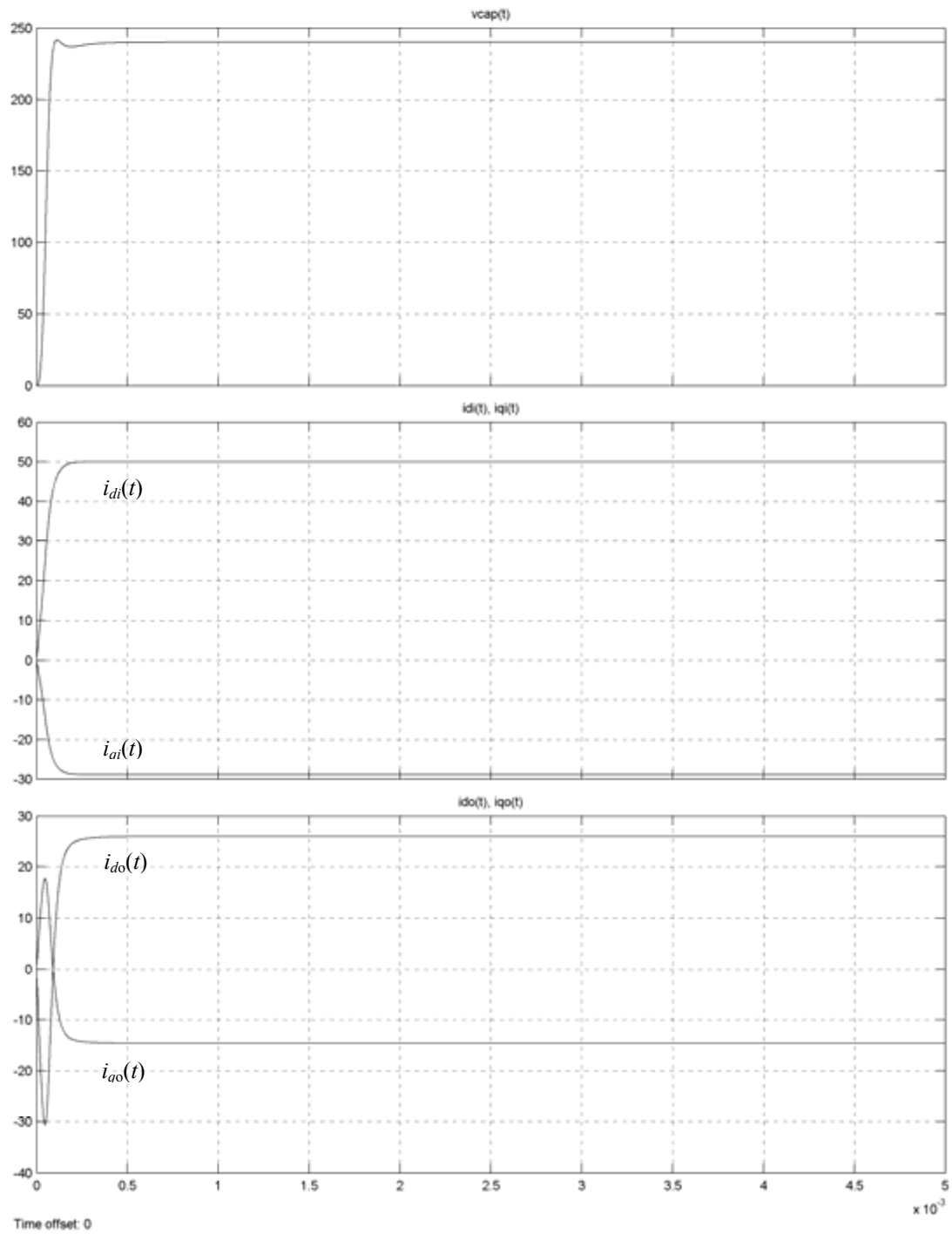
Figure 10.13: Simulation results for the following operating point: Input side: 240 V, 13 Hz, unity power factor Output side: 240 V, 60 Hz, 20 A, unity power factor The first part is the capacitor voltage response, the second part is the input dq currents responses, and the third part is the output dq currents responses
