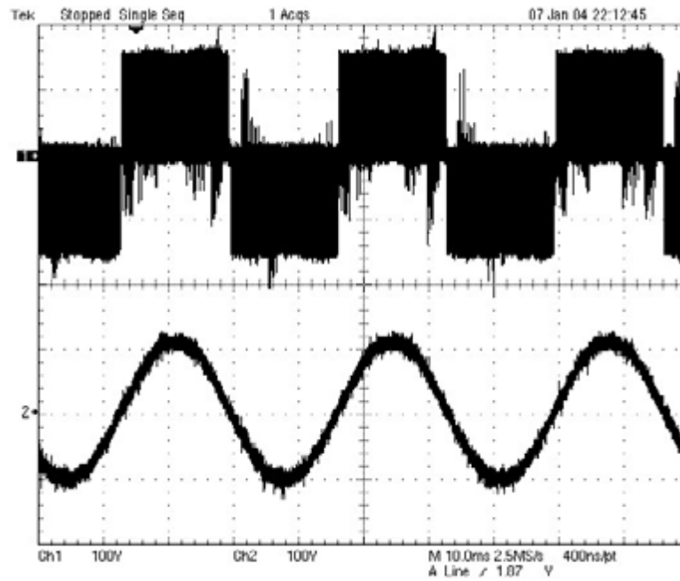
Figure 3.11: The 30-Hz line-line voltage waveforms Trace 1: PWM voltage waveform at the output of the switch network Trace 2: filtered load voltage waveform, after filtered by an LC low-pass network
