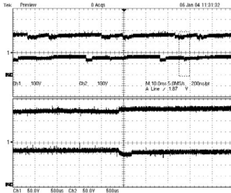
Figure 3.24: The DC capacitor voltage waveforms of two different switch cells. The upper half of the screen illustrates the measured waveforms at 10 ms/div. Trace 1 and Trace 2 are both set to scale of 100 V/div at different ground reference levels. The lower half of the screen shows the same waveforms magnified from the outlined area.
