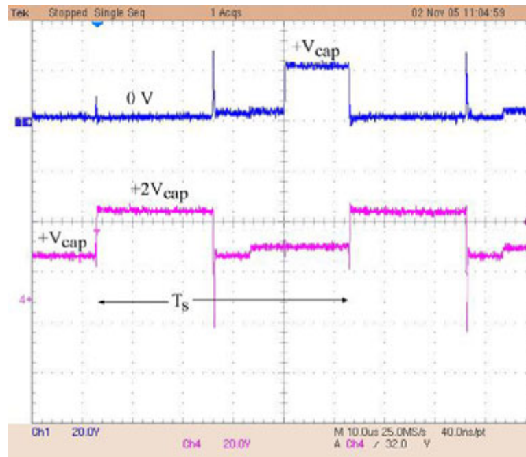
Figure 5.8: Input and output line-line voltage waveforms in one switching period Trace 1: input line-line voltage with two-level switching Trace 4: output line-line voltage with three-level switching
