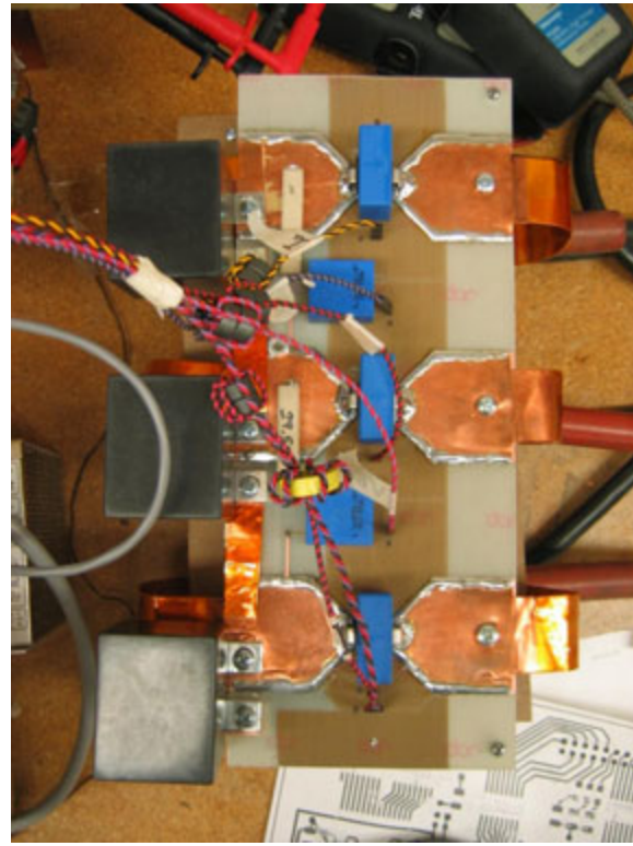
Figure 6.10: Sensor circuits at the output side consist of Hall Effect sensing devices
