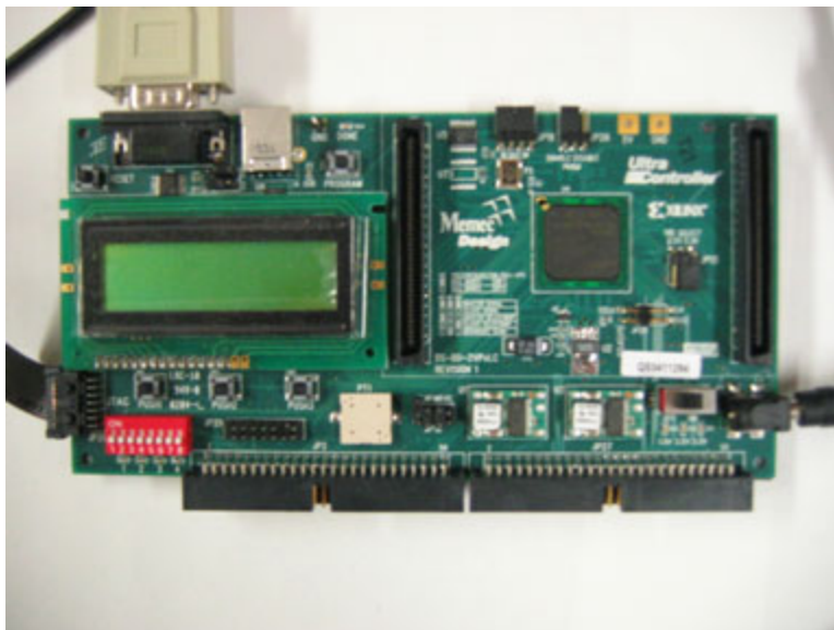
Figure 6.7: Virtex-II Pro XC2VP4 development board
