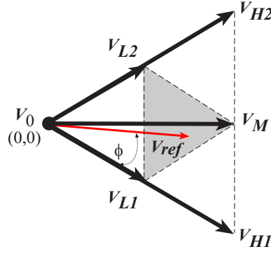
Figure 5.3: SVM for three-level switching, Case 1
