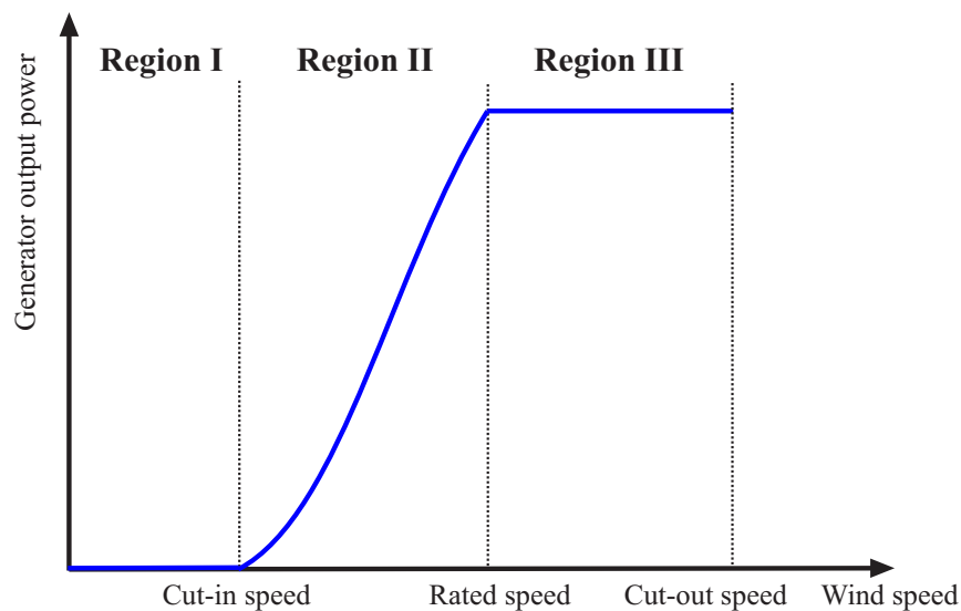
Figure 1.1: Ideal characteristic of a wind turbine generator
