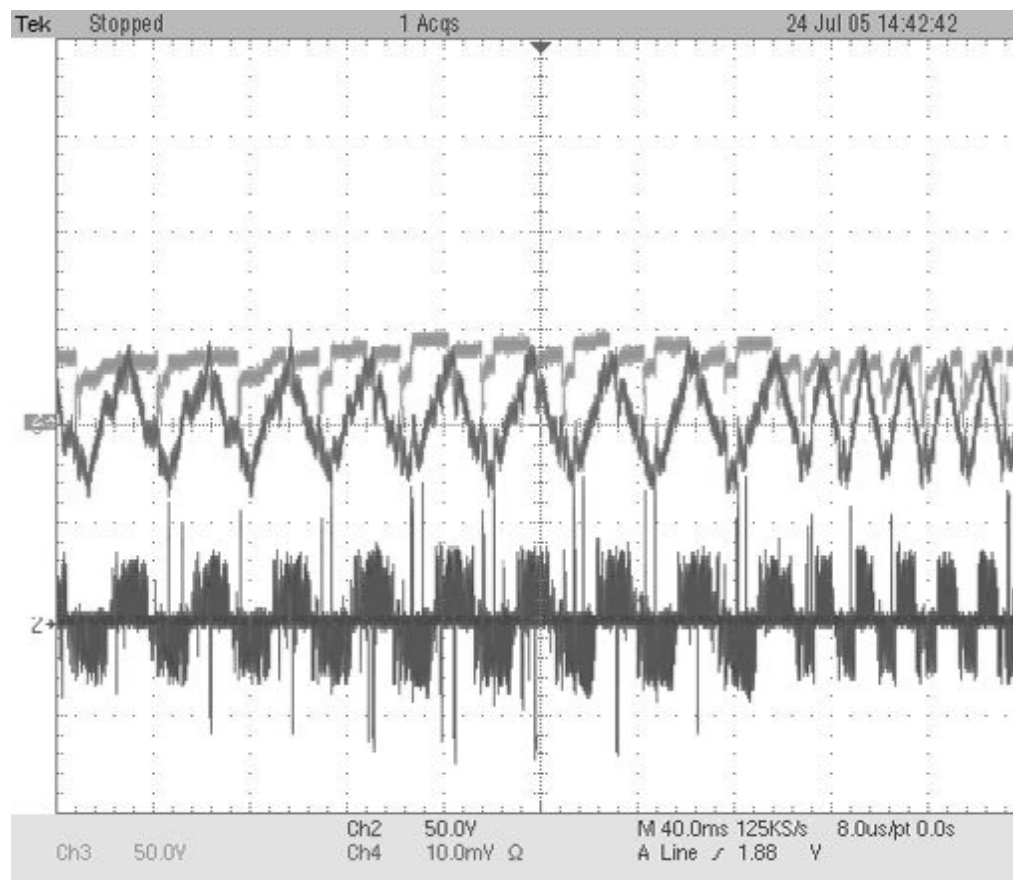
Figure 11.4: Experimental results of the matrix-converter prototype when the output-line frequency changes from 30 Hz to 60 Hz:
