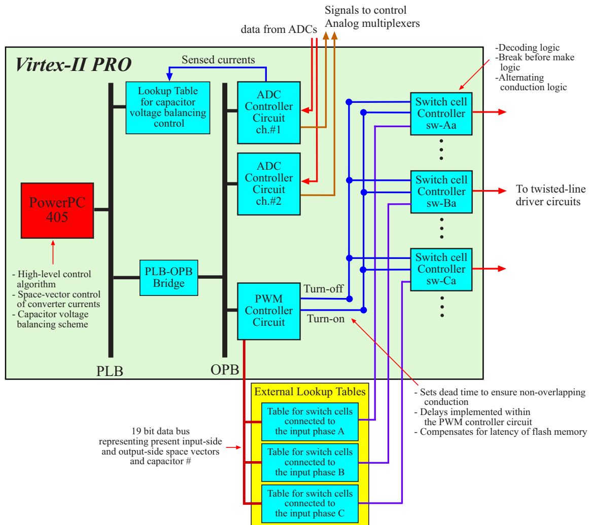
Figure 6.8: Control system block diagram
