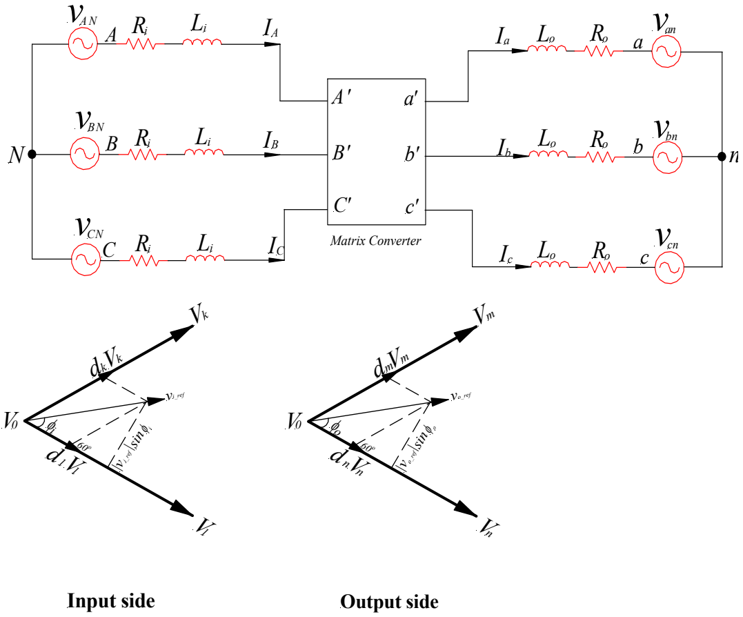
Figure 9.1: Configuration of the matrix converter terminal connections and SVM to control the input and output voltages
