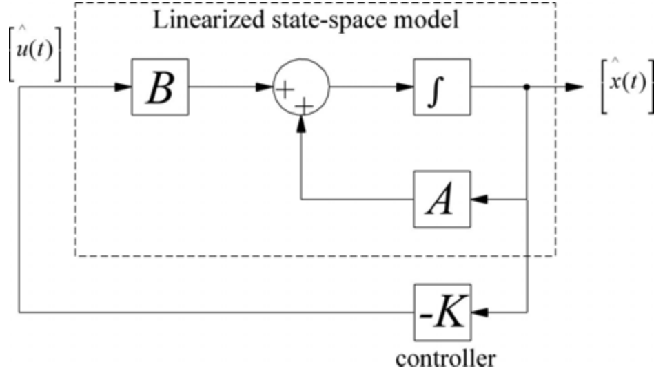
Figure 10.2: State feedback of the linearized model of the matrix converter
