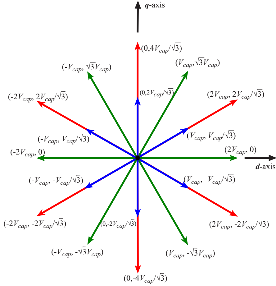
Figure 2.11: The 19 space vectors attainable from the multilevel matrix converter
