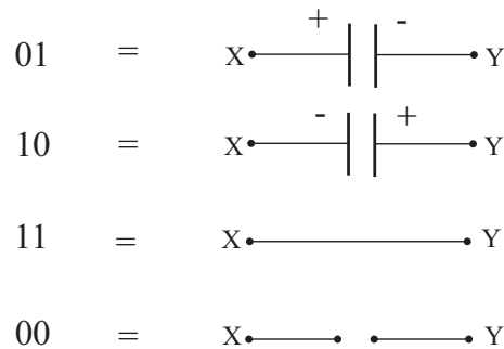
Figure 6.14: Two-bit data representing all four states of switch cell; “X” denotes an input phase and “Y” denotes an output phase
