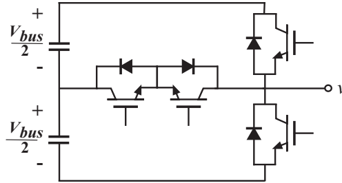
Figure 1.10: Switching device configuration for one phase of a three-level converter with bi-directional switch interconnection
