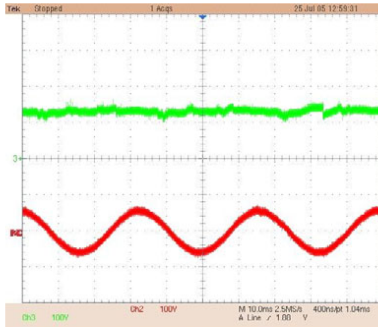
Figure 4.13: Waveforms of a capacitor voltage and a filtered output line-line voltage
