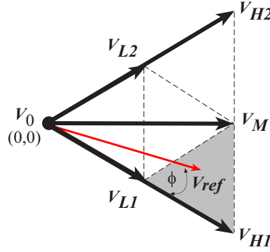
Figure 5.4: SVM for three-level switching, Case 2
