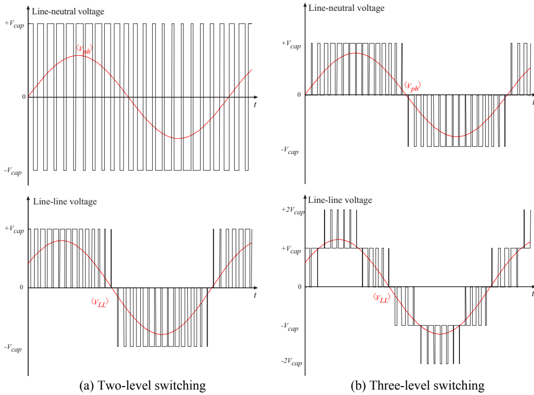
Figure 1.8: Comparison of PWM waveforms for (a) conventional two-level switching and (b) three-level switching
