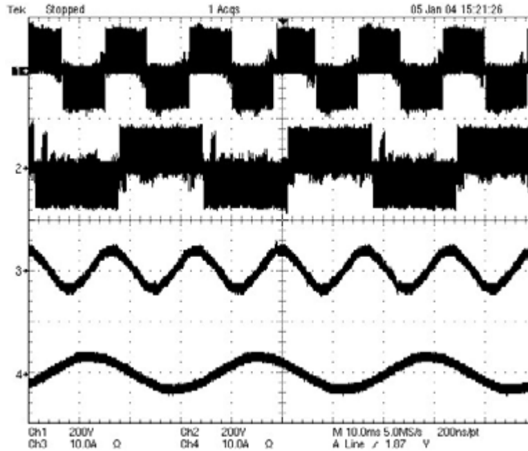
Figure 3.19: Voltage and current waveforms. Case 1 Trace 1: input PWM line-line voltage waveform at 200 V/div Trace 2: output PWM line-line voltage waveform at 200 V/div Trace 3: input phase current at 10 A/div Trace 4: output phase current at 10 A/div Horizontal scale: 10 ms/div
