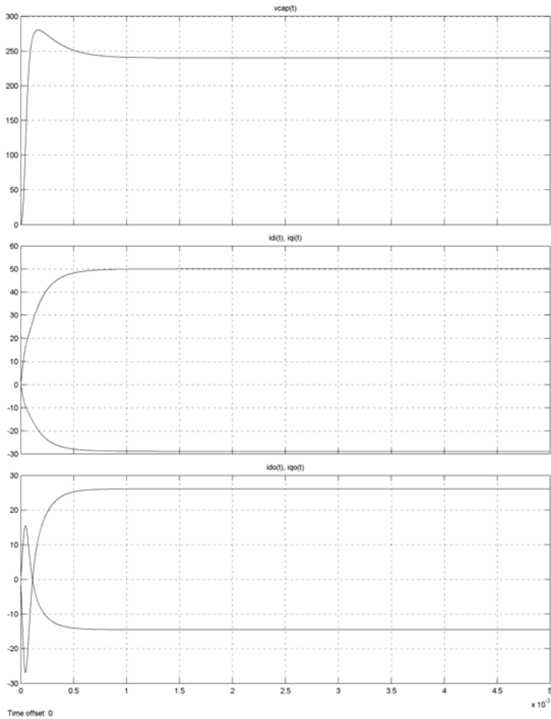
Figure 10.7: Simulation results for the following operating point: Input side: 240 V, 13 Hz, unity power factor Output side: 240 V, 60 Hz, 20 A, unity power factor The first part is the capacitor voltage response, the second part is the input dq currents responses, and the third part is the output dq currents responses
