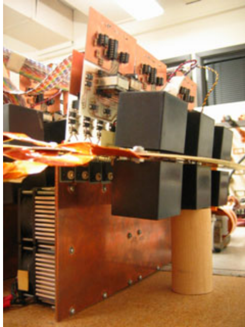
Figure 6.5: Side view of a PCB, showing the IGBTs mounted to the heat sinks through the copper heat spreader
