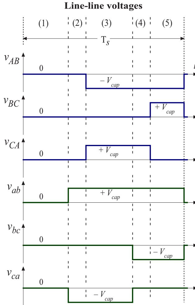
Figure 3.6: PWM line-line voltages in the given switching period for the example
