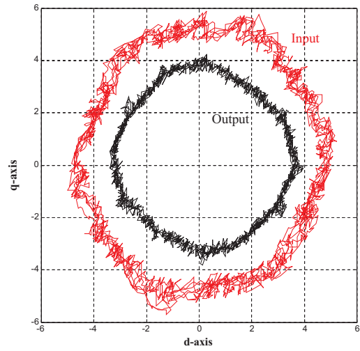
Figure 3.32: Trajectories of input- and output-currents in dq coordinate
