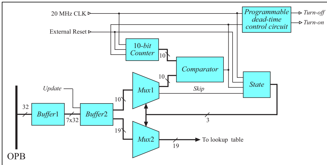
Figure 6.13: Block diagram of the PWM controller circuit
