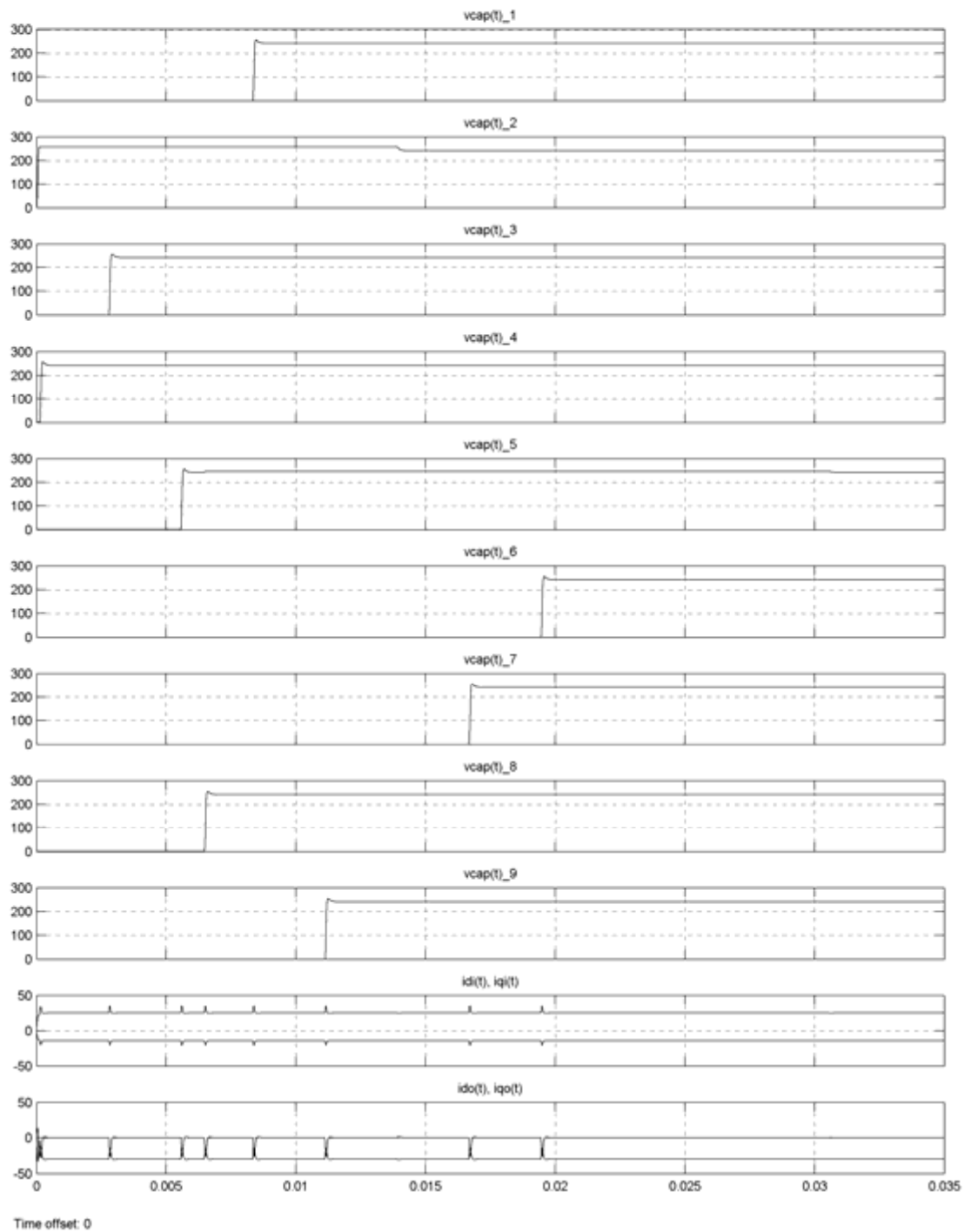
Figure 10.20: Simulation results for the following operating point: Input side: 240 V, 13 Hz, unity power factor Output side: 240 V, 60 Hz, 20 A, 0.5 power factor The first nine parts are the capacitor voltages responses, the tenth part is the input dq currents responses, and the last part is the output dq currents responses
