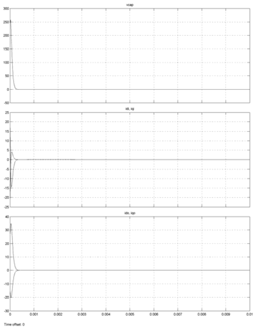
Figure 10.10: Simulation results of the closed-loop linearized state-space model of the matrix converter when an optimal controller is used
