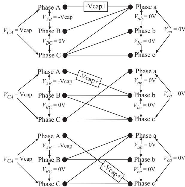
Figure 4.5: An example of redundant switching combinations having the input current I_A through switchcell capacitors
