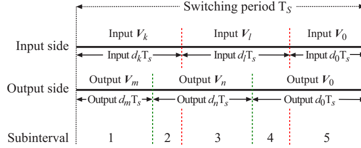
Figure 3.3: SVM of both input and output sides, dividing the switching period into five subintervals
