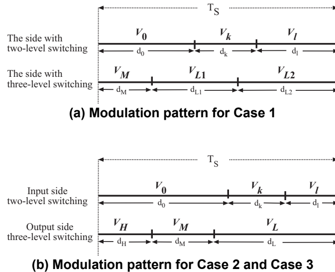
Figure 5.6: Modulation patterns in one switching period for three-level switching
