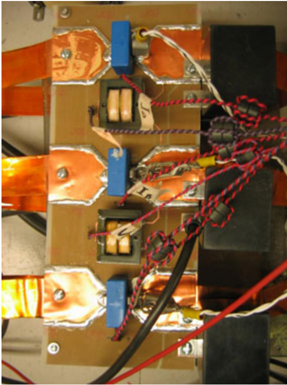
Figure 6.9: Sensor circuits at the input side consist of transformers and Hall Effect sensing devices
