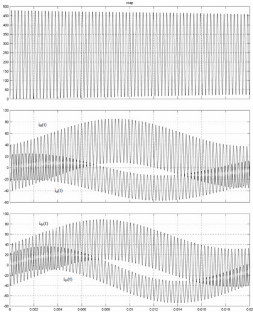
Figure 10.1: Output response example of the matrix converter nonlinear model. The parameters are Input side: 25 Hz, unity power factor Output side: 240 V (line-to-line), 20 A, 60 Hz, 0.95 power factor
