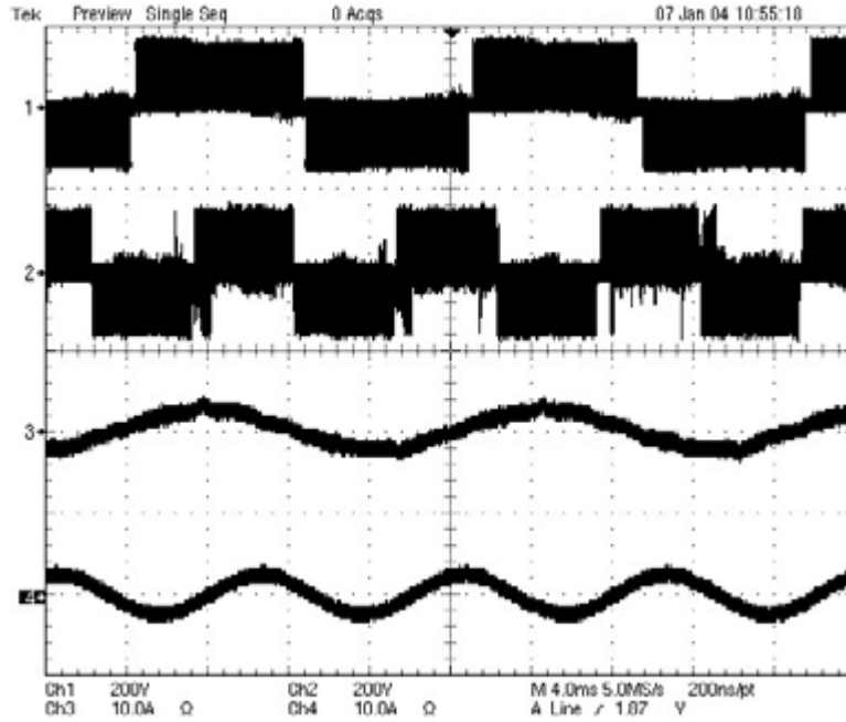
Figure 3.25: Voltage and current waveforms, Case 2 Trace 1: input line-line PWM voltage waveform at 200 V/div Trace 2: output line-line PWM voltage waveform at 200 V/div Trace 3: input phase current at 10 A/div Trace 4: output phase current at 10 A/div. Horizontal scale: 4 ms/div
