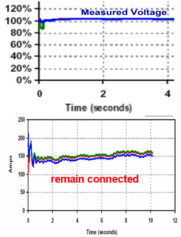
Figure 3: Measurements at the point of interconnection during the fault event. a) Voltage traces b) Current traces.
