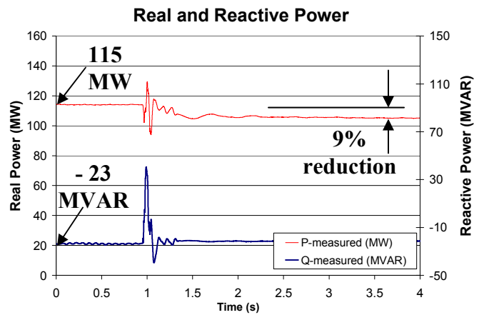
Figure 7. Real and reactive power measured at the POI.
