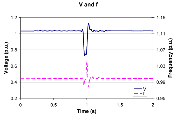
Figure 6 Per unit voltage and frequency during the fault.
