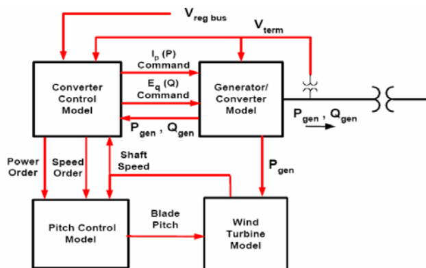
Figure 3. Block diagram of WECC generic DFAG model.
