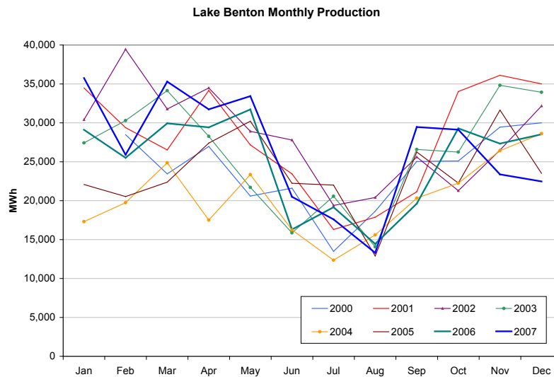
Figure 1. Monthly production of Lake Benton wind power plant.
