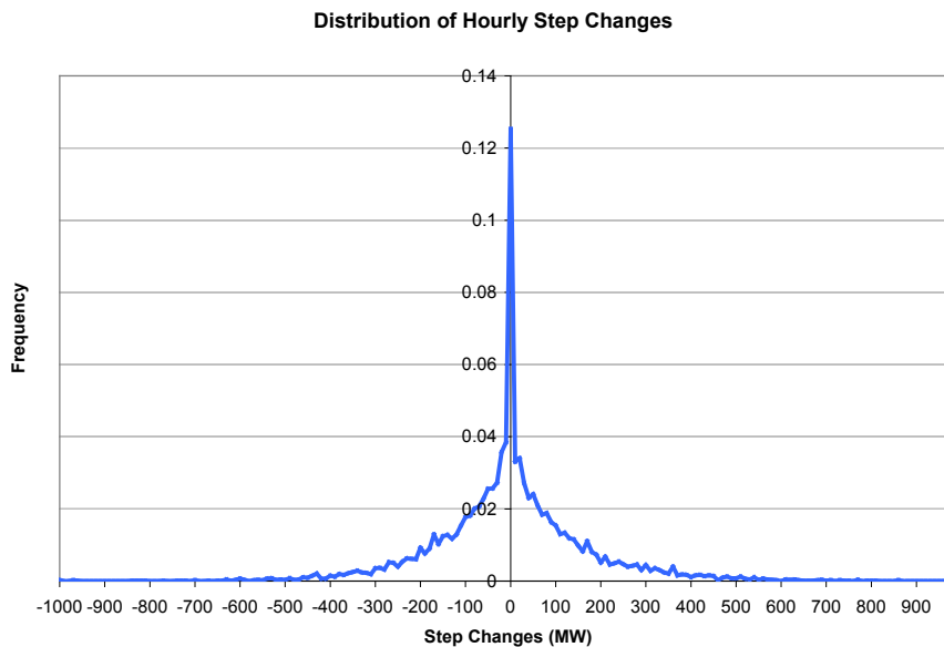
Figure 3. Distribution of hourly wind power changes.
