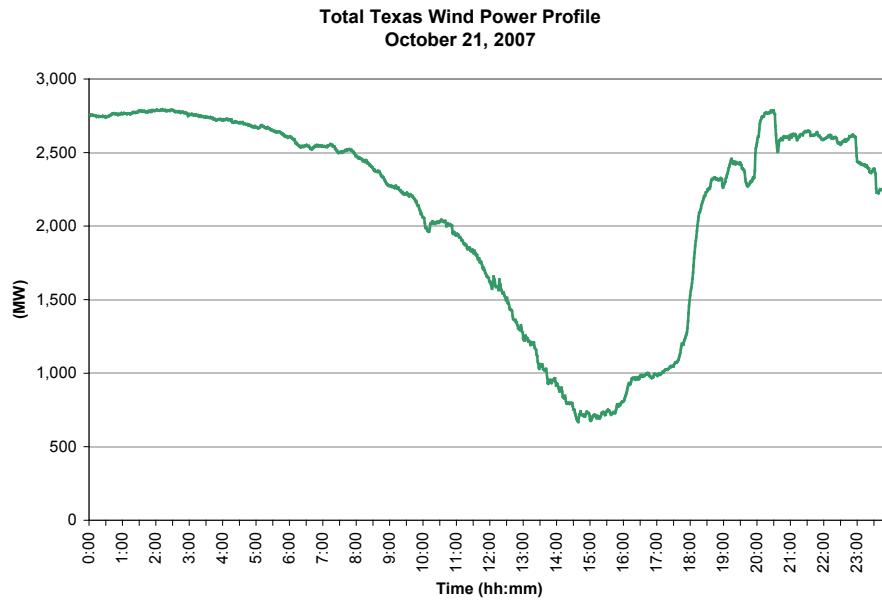
Figure 4. Daily 1-minute average power profile.
