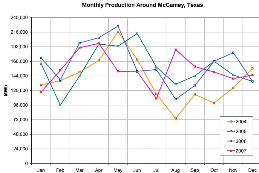
Figure 2. Monthly production of wind plants near McCamey, Texas.
