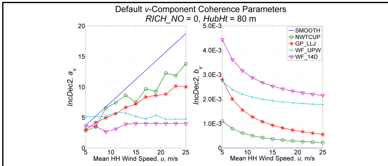
Figure 14. Default v -component coherence parameters, IncDec2 , ( a_v left, b_v right) as a function of wind speed, using RICH_NO = 0 and HubHt = 80 m (IEC does not define v -component coherence parameters)
