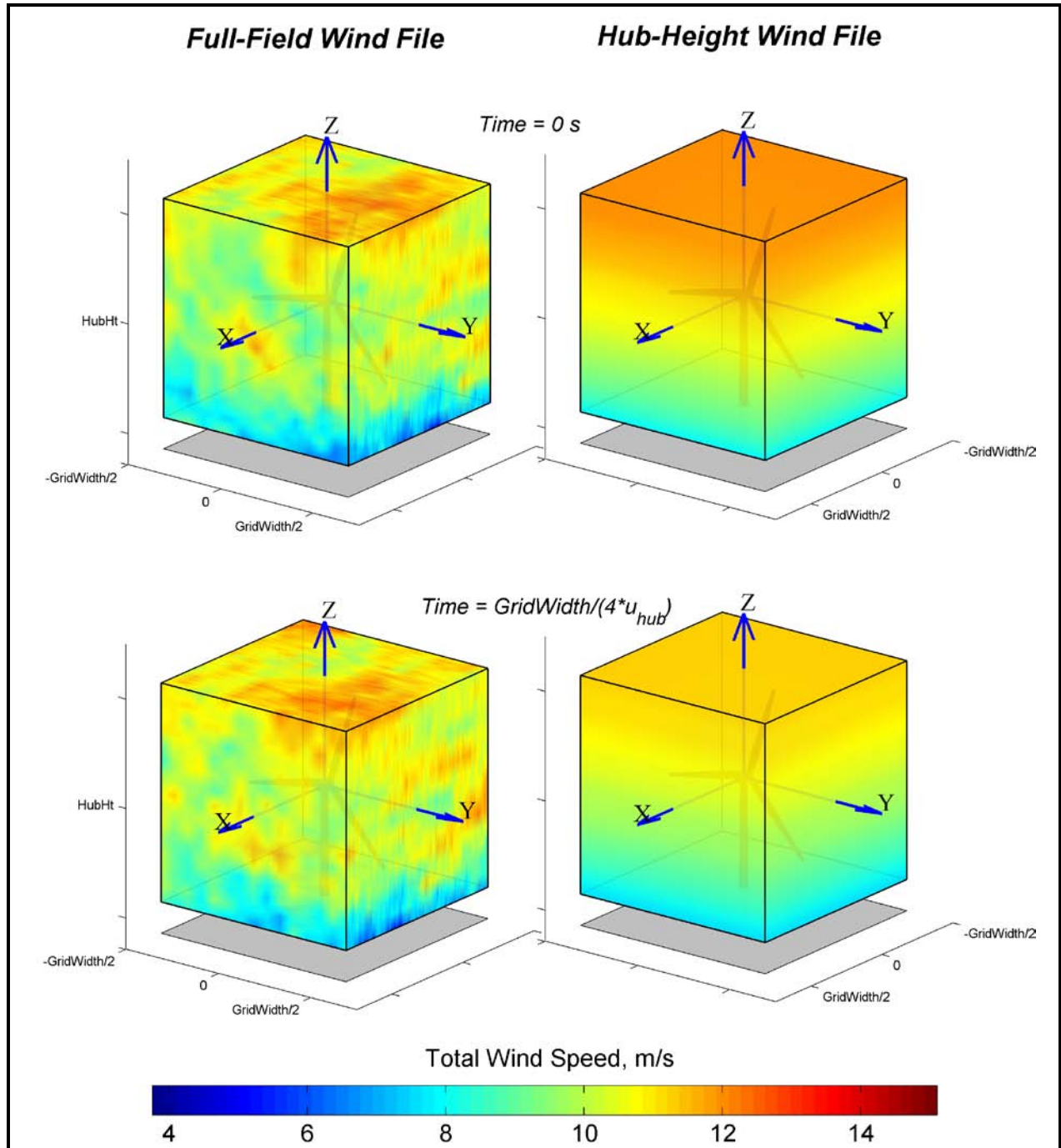
Figure 17. Example TurbSim FF and HH wind files as implemented in AeroDyn. The bottom left plot shows the FF grids after marching GridWidth/4 meters (along positive X ) from the position in the upper left plot; HH wind files (right column) do not march through the turbine. At each time step, the FF wind velocity at X = GridWidth/2, Y = 0, Z = HubHt is identical to the HH wind velocity at X = 0, Y = 0, Z = HubHt . Because TurbSim sets the horizontal shear to 0 in the HH files, the velocity does not change with either X or Y . Thus, the wind velocities in the FF and HH files are identical at X = GridWidth/2, Y = 0, Z = HubHt (where the X axis on the plots emerges from the wind volume).
